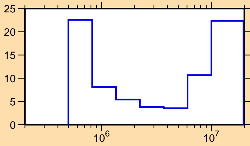
\Delta\sigma/\sigma vs. E for ^{164}\text{Ho}(n,n\text{cont.})
