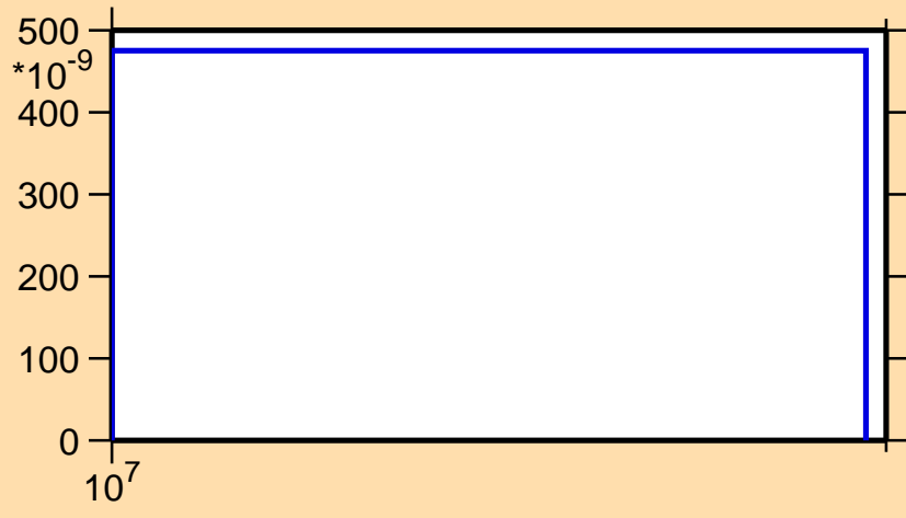
\sigma vs. E for ^{164}\text{Ho}(n,\text{nd})
