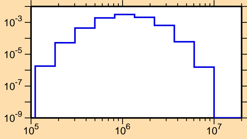
\sigma vs. E for ^{164}\text{Ho}(n,n_3)
