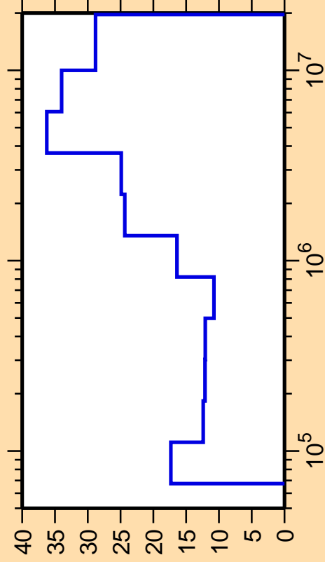
\Delta\sigma/\sigma vs. E for ^{164}\text{Ho}(n,n_2)
