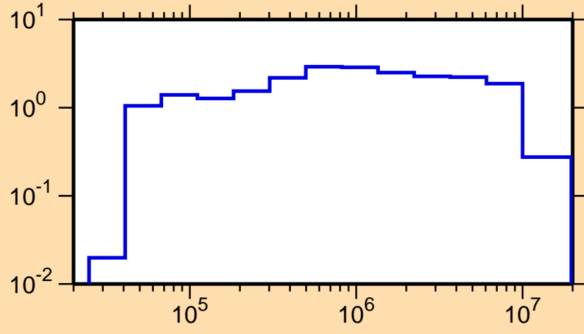
\sigma vs. E for ^{164}\text{Ho}(n,\text{inel.})
