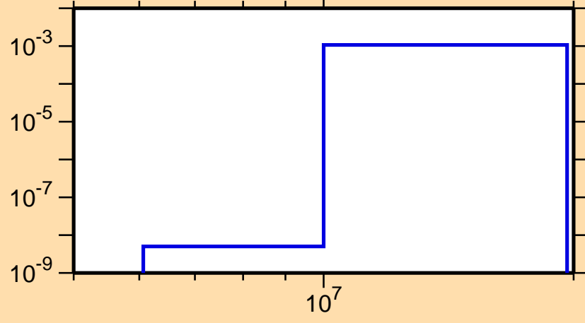
\sigma vs. E for ^{164}\text{Ho}(n,np)
