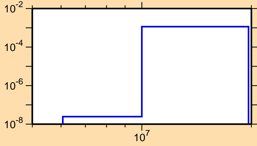
\sigma vs. E for ^{164}\text{Ho}(n,d)
