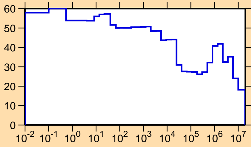
\Delta\sigma/\sigma vs. E for ^{164}\text{Ho}(n,p)
