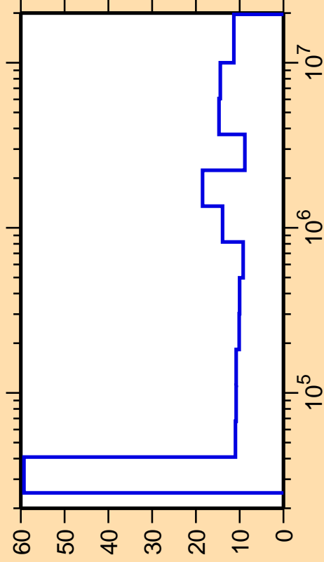
\Delta\sigma/\sigma vs. E for ^{164}\text{Ho}(n,n_1)
