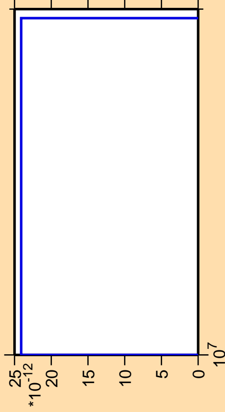
\Delta\sigma/\sigma vs. E for ^{164}\text{Ho} (mt 11)
