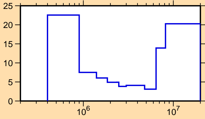
\Delta\sigma/\sigma vs. E for ^{164}\text{Ho}(n,n\text{cont.})
