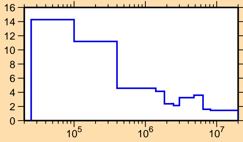
\Delta\sigma/\sigma vs. E for ^{164}\text{Ho}(n,\text{tot.})
