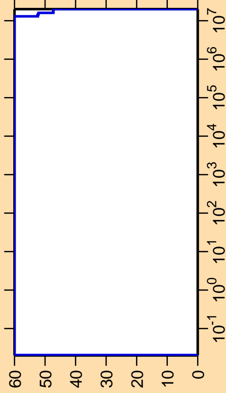
\Delta\sigma/\sigma vs. E for ^{164}\text{Ho}(n,\alpha)
