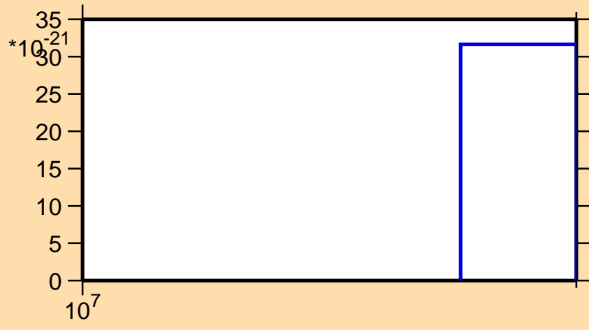
\sigma vs. E for ^{166}\text{Ho} (mt 11)
