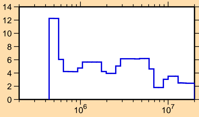
\Delta\sigma/\sigma vs. E for ^{166}\text{Ho}(n, el.)
