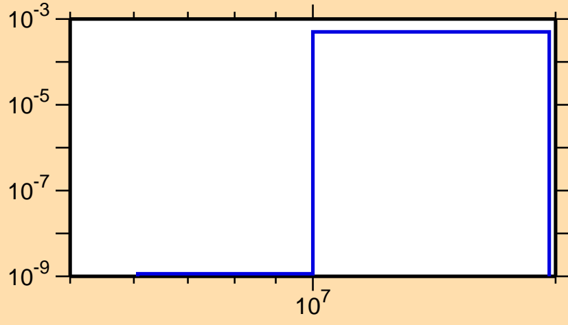
\sigma vs. E for ^{166}\text{Ho}(n,d)
