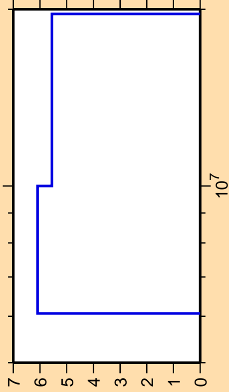
\Delta\sigma/\sigma vs. E for ^{166}\text{Ho}(n,2n)
