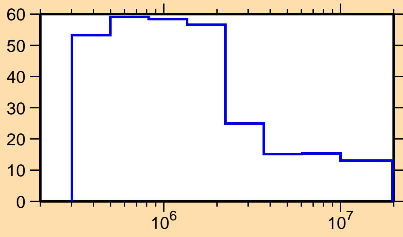
\Delta\sigma/\sigma vs. E for ^{166}\text{Ho}(n,n_1)
