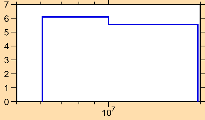
\Delta\sigma/\sigma vs. E for ^{166}\text{Ho}(n,2n)
