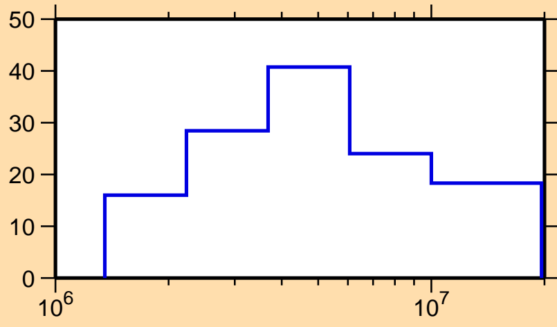
\Delta\sigma/\sigma vs. E for ^{166}\text{Ho}(n,p)
