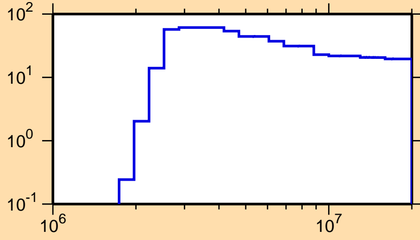
\Delta\sigma/\sigma vs. E for ^{166}\text{Ho}(n,p)
