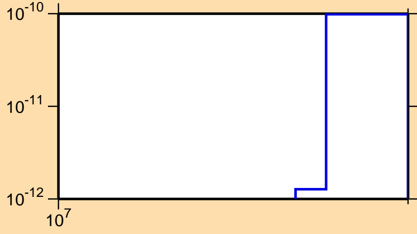
\sigma vs. E for ^{166}\text{Ho}(n,\text{He3})
