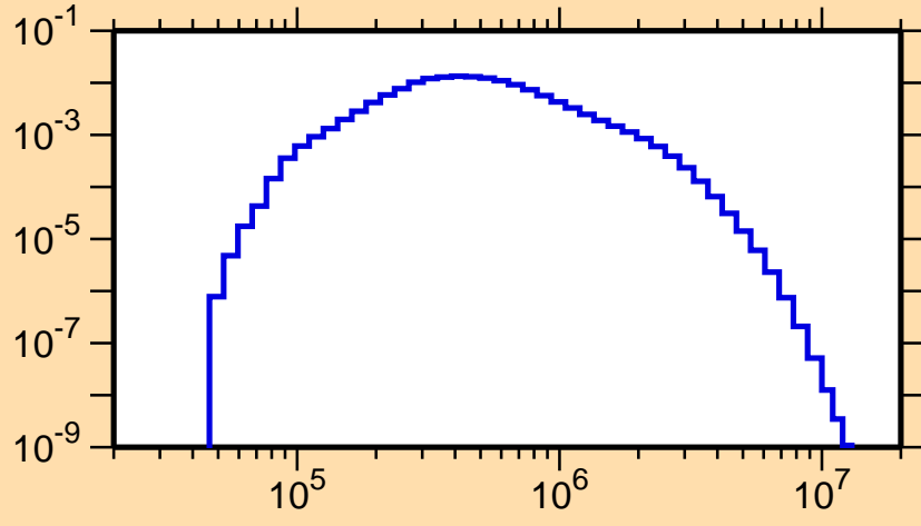
\sigma vs. E for ^{166}\text{Ho}(n,n_2)
