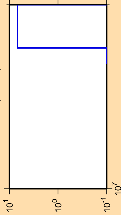
\Delta\sigma/\sigma vs. E for ^{167}\text{Ho}(n,\text{He3})
