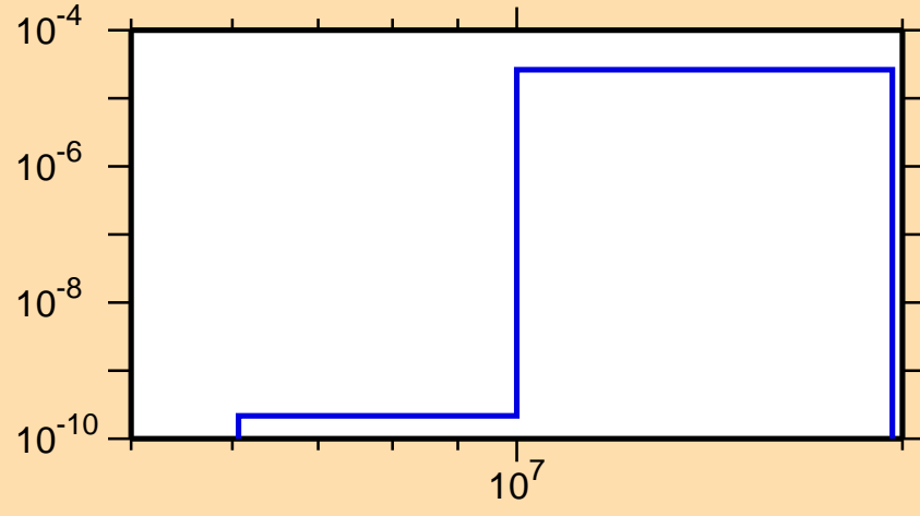
\sigma vs. E for ^{167}\text{Ho}(n,n\alpha)
