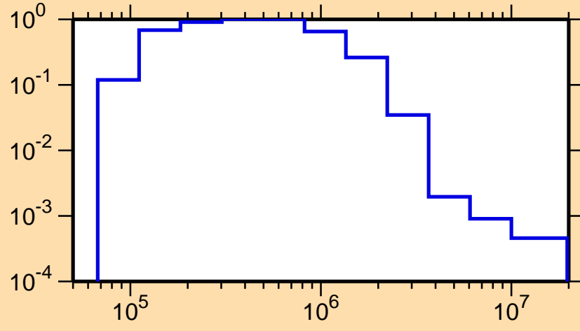
\sigma vs. E for ^{167}\text{Ho}(n,n_1)
