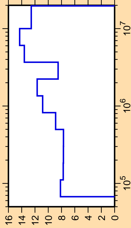
\Delta\sigma/\sigma vs. E for ^{167}\text{Ho}(n,n_1)
