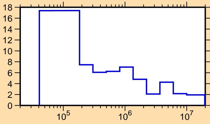
\Delta\sigma/\sigma vs. E for ^{168}\text{Ho}(n,\text{tot.})
