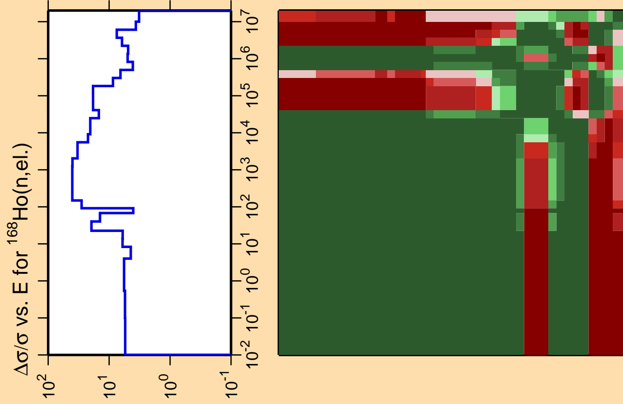
Correlation Matrix
