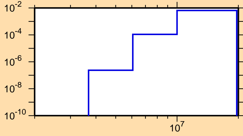
\sigma vs. E for ^{168}\text{Ho}(n,p)
