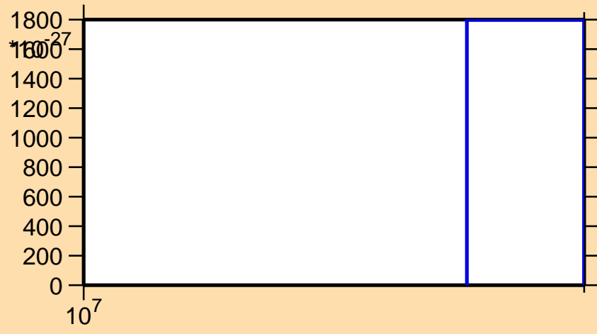
\sigma vs. E for ^{168}\text{Ho} (mt 42)
