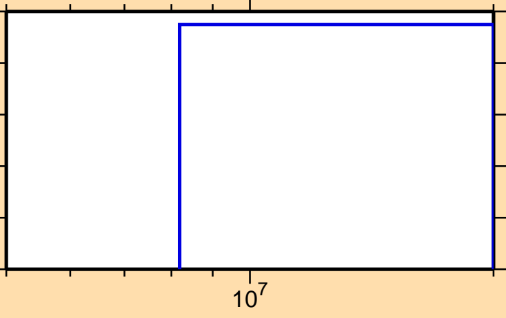
\sigma vs. E for ^{168}\text{Ho}(n,\text{He3})
