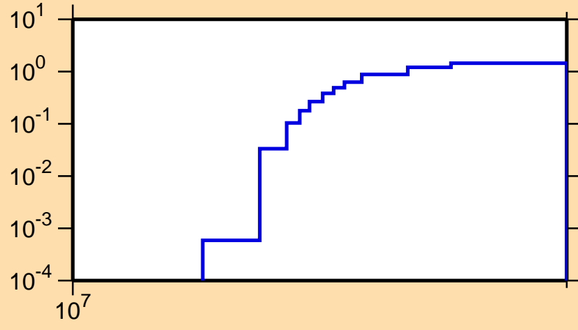
\sigma vs. E for ^{169}\text{Ho}(n,3n)
