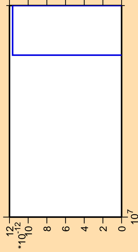
\Delta\sigma/\sigma vs. E for ^{169}\text{Ho} (mt 42)
