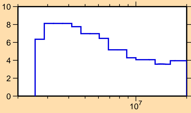
\Delta\sigma/\sigma vs. E for ^{169}\text{Ho}(n,\text{nonel.})
