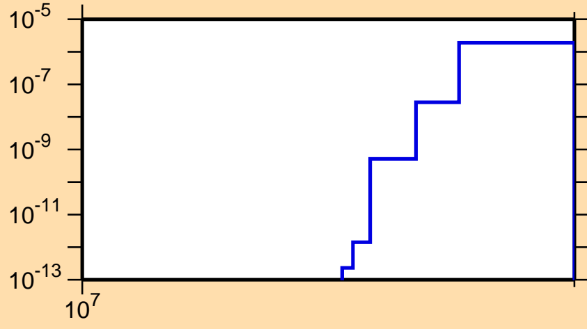
\sigma vs. E for ^{169}\text{Ho}(n,nt)
