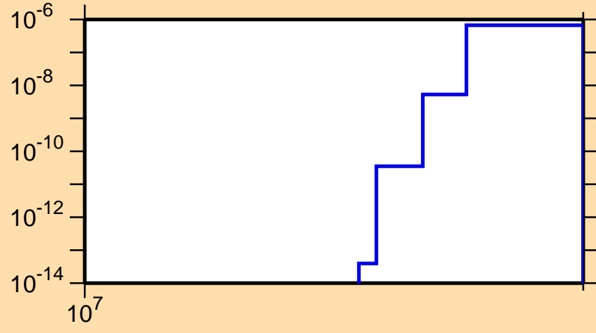
\sigma vs. E for ^{169}\text{Ho}(n,\text{nd})
