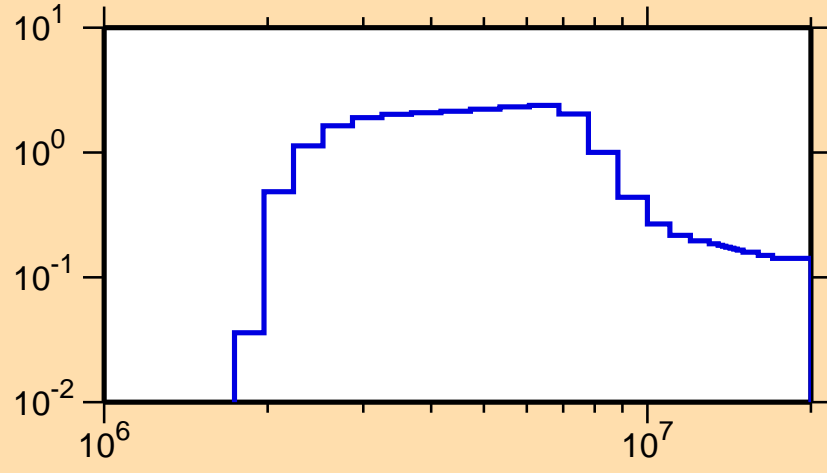
\sigma vs. E for ^{169}\text{Ho}(n,n\text{cont.})
