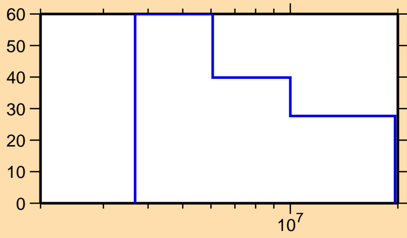
\Delta\sigma/\sigma vs. E for ^{169}\text{Ho}(n,p)
