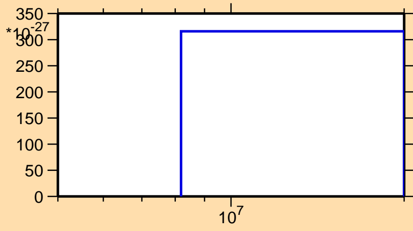
\sigma vs. E for ^{169}\text{Ho} (mt 42)
