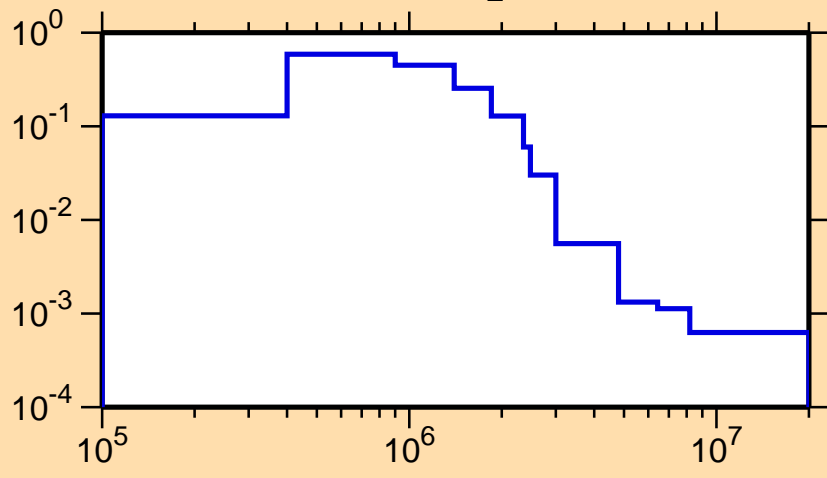
\sigma vs. E for ^{169}\text{Ho}(n,n_2)
