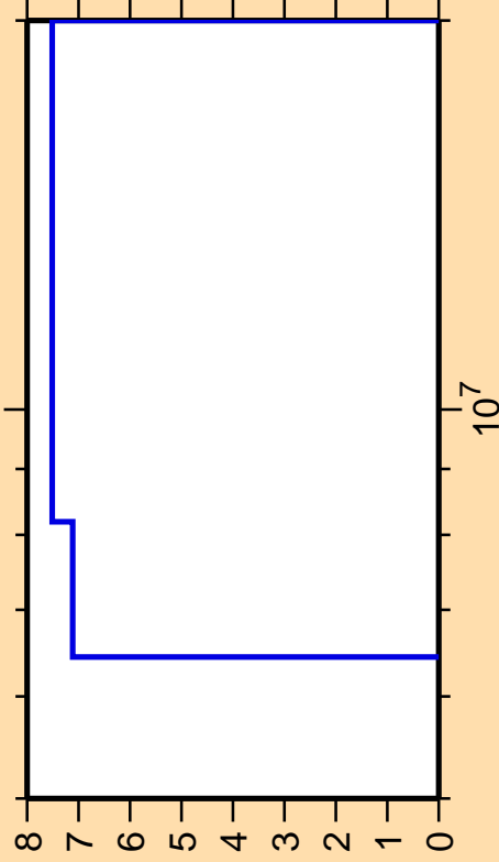
\Delta\sigma/\sigma vs. E for ^{169}\text{Ho}(n,2n)
