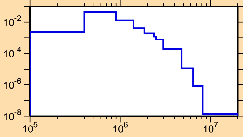
\sigma vs. E for ^{170}\text{Ho}(n,n_3)
