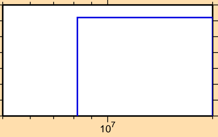
\sigma vs. E for ^{170}\text{Ho}(n,nt)
