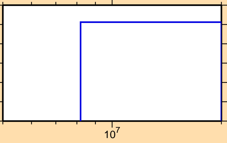
\sigma vs. E for ^{170}\text{Ho}(n,t)
