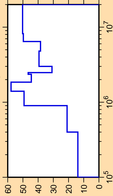
\Delta\sigma/\sigma vs. E for ^{170}\text{Ho}(n,n_3)
