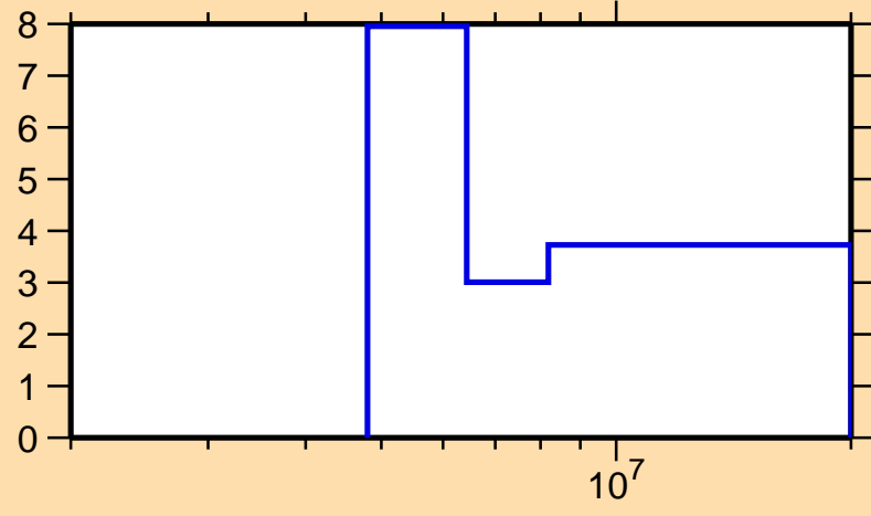
\Delta\sigma/\sigma vs. E for ^{170}\text{Ho}(n,\text{el.})
