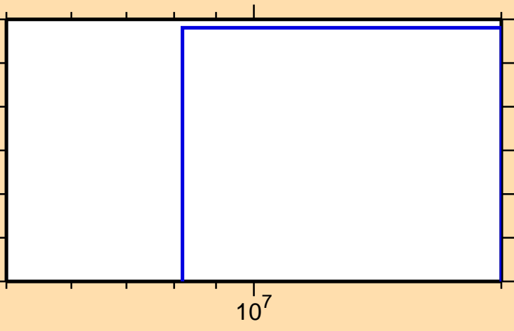
\sigma vs. E for ^{170}\text{Ho}(n,n\alpha)
