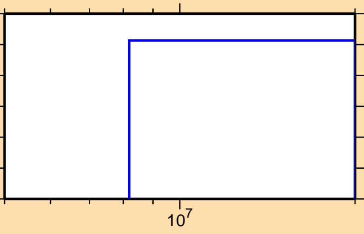
\sigma vs. E for ^{170}\text{Ho}(n,2np)
