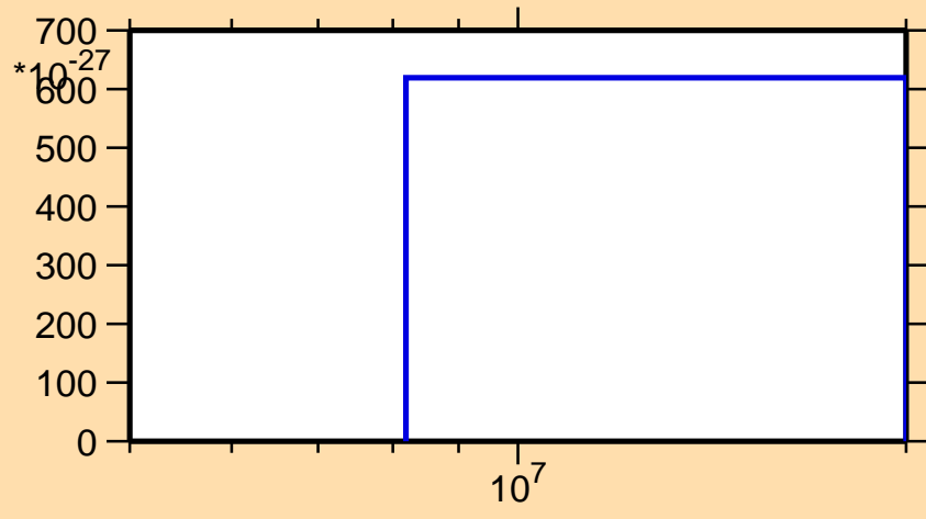
\sigma vs. E for ^{170}\text{Ho} (mt 42)
