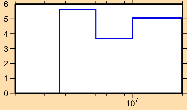
\Delta\sigma/\sigma vs. E for ^{171}\text{Ho}(n,\text{nonel.})
