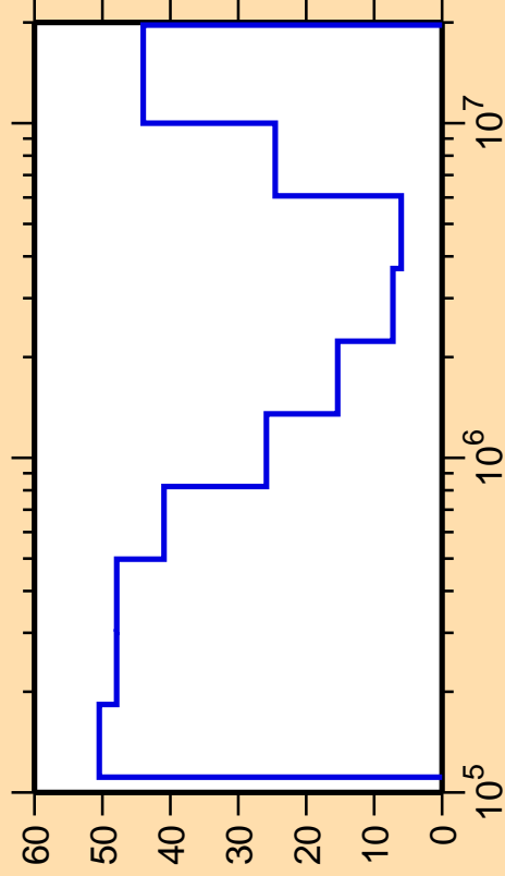
\Delta\sigma/\sigma vs. E for ^{171}\text{Ho}(n,n\text{cont.})
