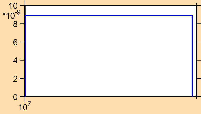
\sigma vs. E for ^{171}\text{Ho}(n,\text{nd})
