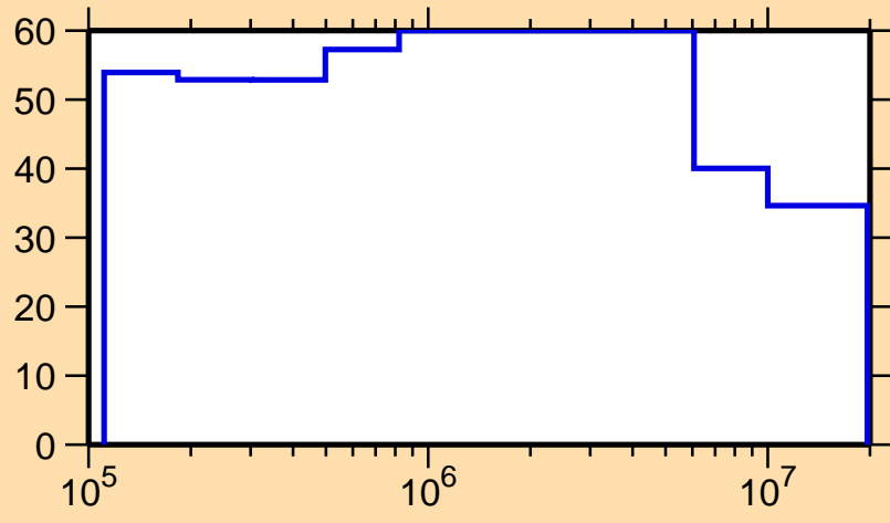
\Delta\sigma/\sigma vs. E for ^{171}\text{Ho}(n,n_1)
