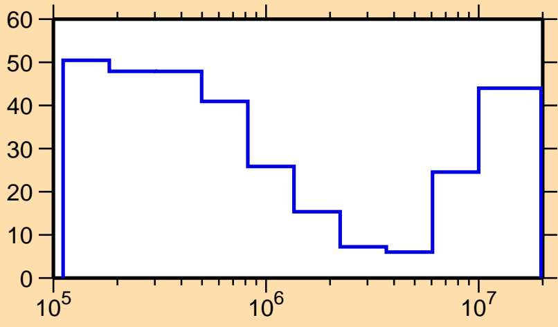
\Delta\sigma/\sigma vs. E for ^{171}\text{Ho}(n,n\text{cont.})
