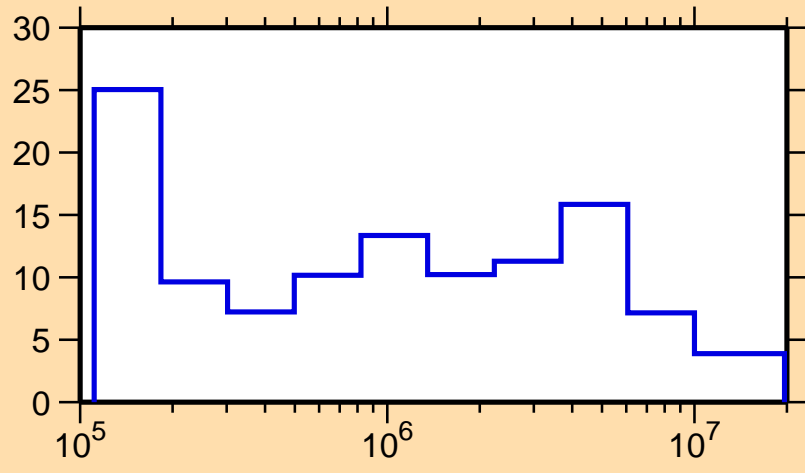
\Delta\sigma/\sigma vs. E for ^{171}\text{Ho}(n,\text{el.})
