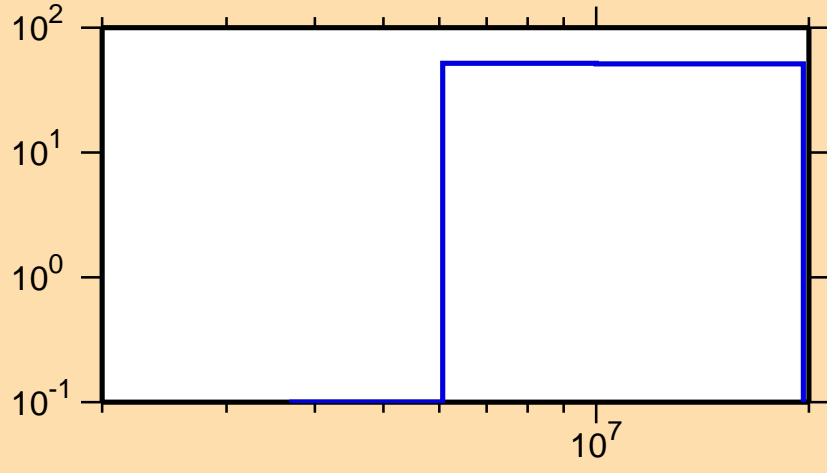
\Delta\sigma/\sigma vs. E for ^{171}\text{Ho}(n,p)
