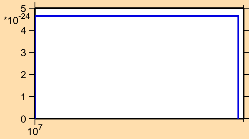
\sigma vs. E for ^{171}\text{Ho} (mt 42)
