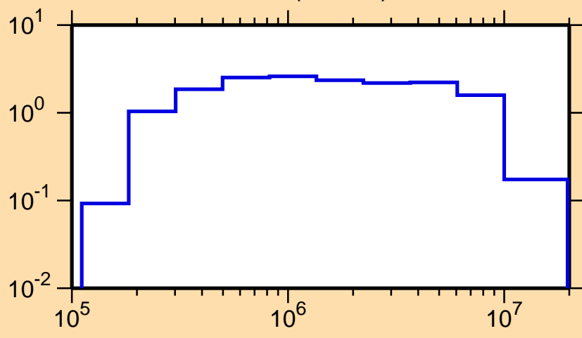
\sigma vs. E for ^{171}\text{Ho}(n,\text{inel.})
