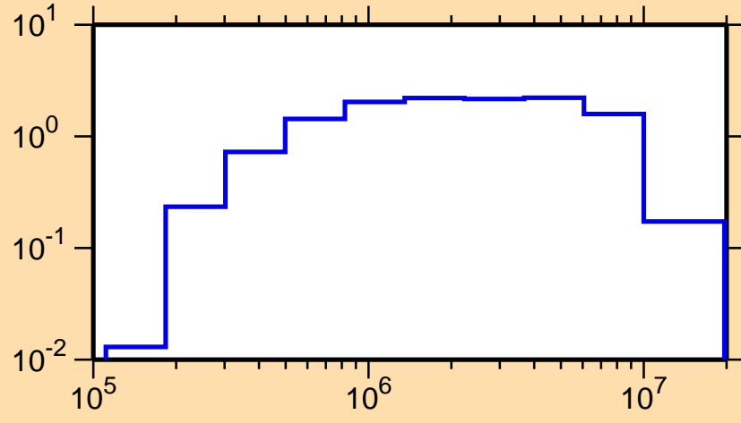
\sigma vs. E for ^{171}\text{Ho}(n,n\text{cont.})
