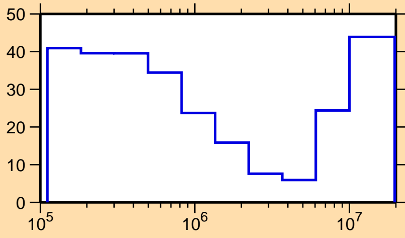
\Delta\sigma/\sigma vs. E for ^{171}\text{Ho}(n,\text{inel.})
