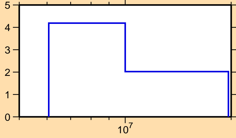
\Delta\sigma/\sigma vs. E for ^{171}\text{Ho}(n,\text{tot.})
