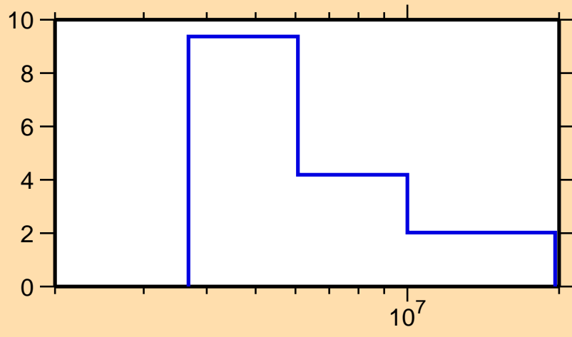
\Delta\sigma/\sigma vs. E for ^{171}\text{Ho}(n,\text{tot.})
