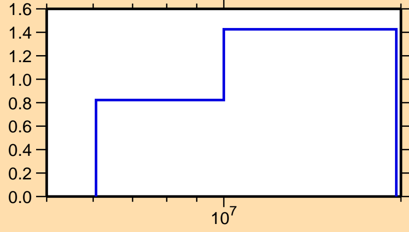
\sigma vs. E for ^{171}\text{Ho}(n,2n)
