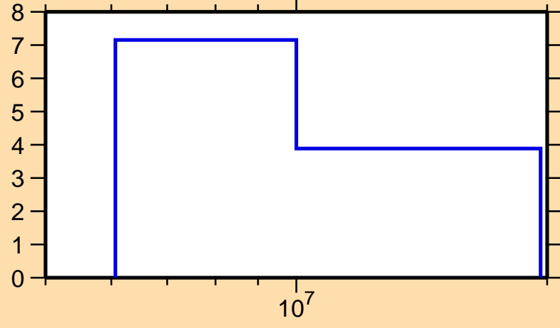
\Delta\sigma/\sigma vs. E for ^{171}\text{Ho}(n,\text{el.})
