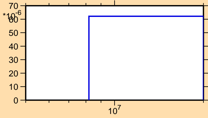
\sigma vs. E for ^{171}\text{Ho}(n,d)
