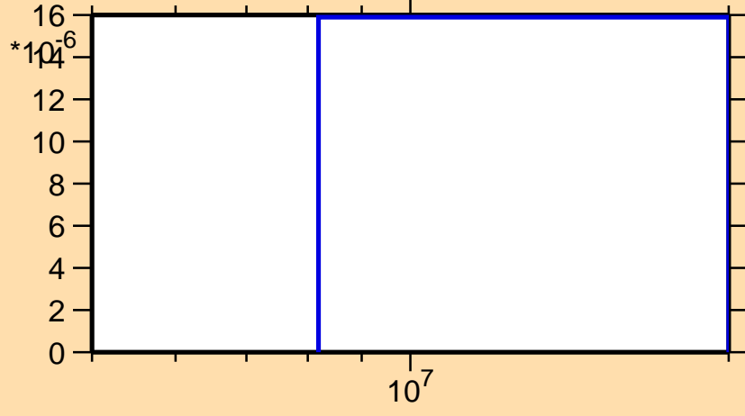
\sigma vs. E for ^{171}\text{Ho}(n,t)
