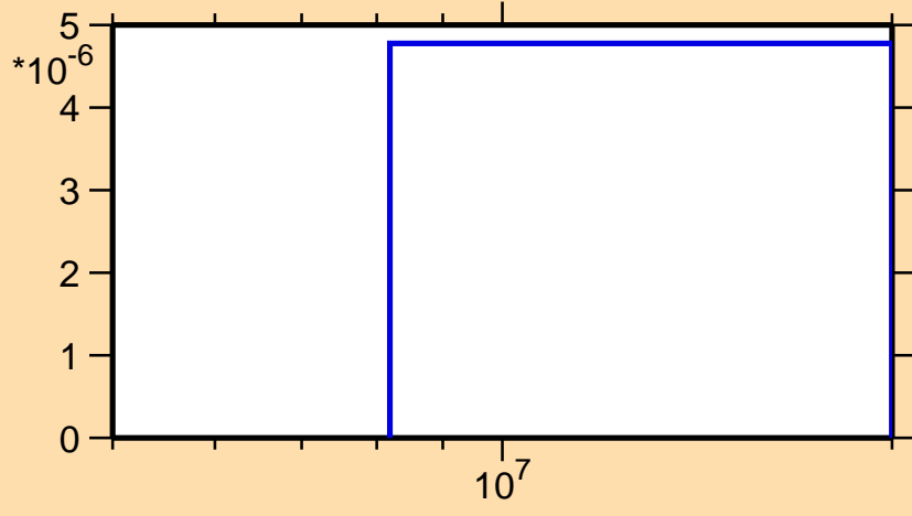
\sigma vs. E for ^{171}\text{Ho}(n,n\alpha)
