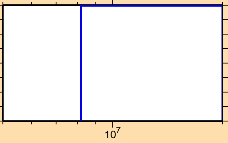
\sigma vs. E for ^{171}\text{Ho}(n,t)
