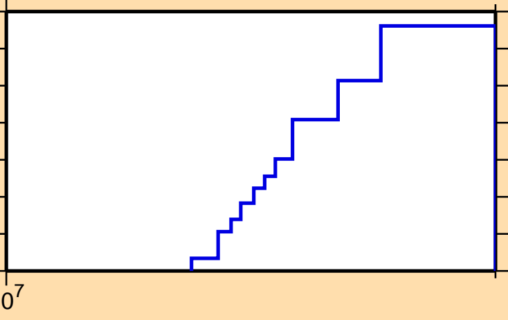
\sigma vs. E for ^{172}\text{Ho}(n,2n\alpha)
