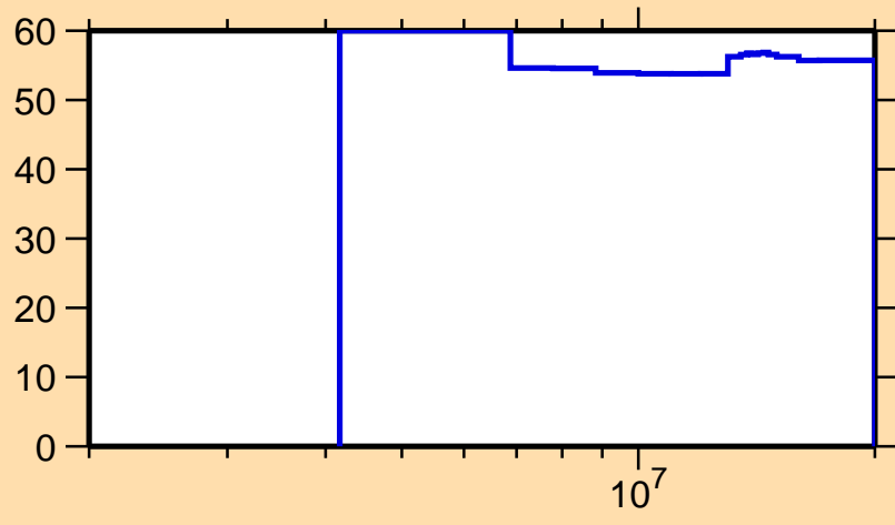
\Delta\sigma/\sigma vs. E for ^{172}\text{Ho}(n,\gamma)
