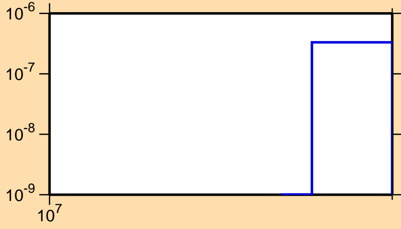
\sigma vs. E for ^{172}\text{Ho}(n,2np)
