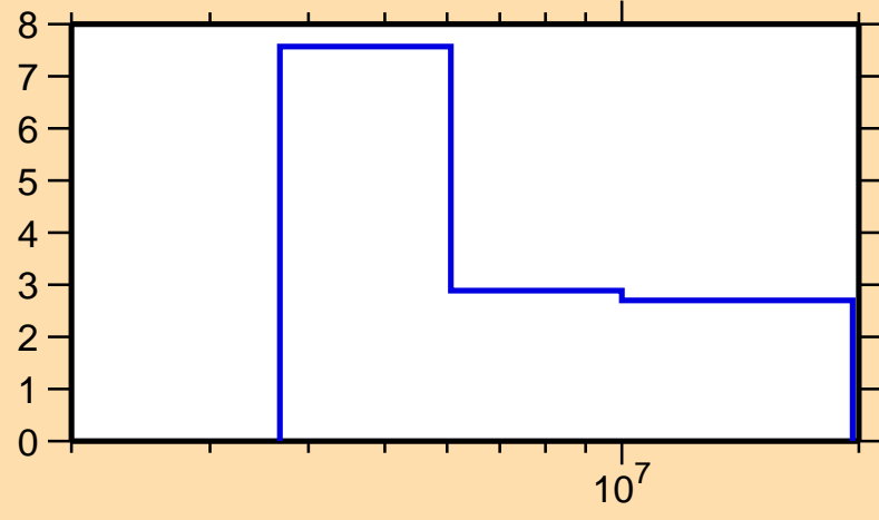
\Delta\sigma/\sigma vs. E for ^{172}\text{Ho}(n,\text{tot.})
