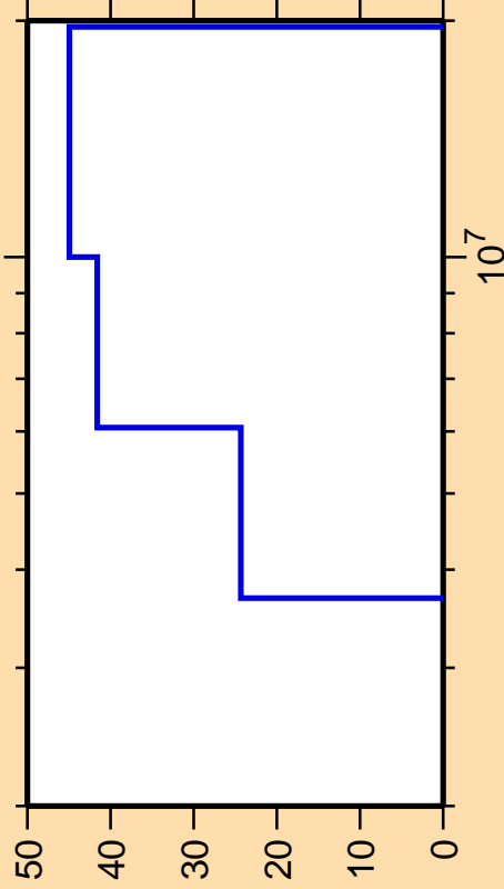
\Delta\sigma/\sigma vs. E for ^{172}\text{Ho}(n,n\text{cont.})
