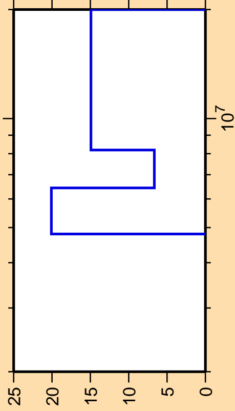
\Delta\sigma/\sigma vs. E for ^{172}\text{Ho}(n,2n)
