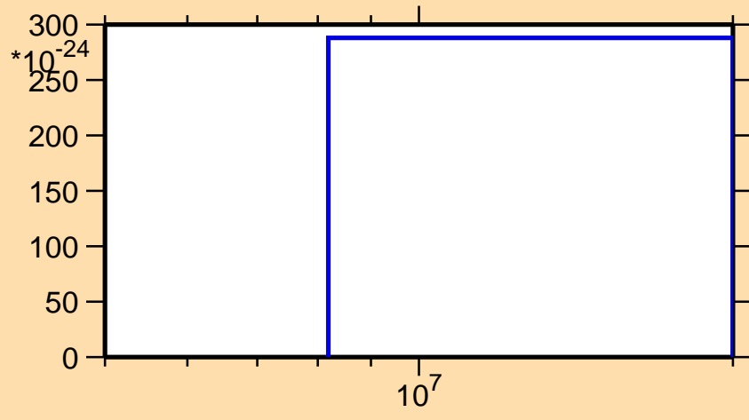
\sigma vs. E for ^{172}\text{Ho} (mt 42)
