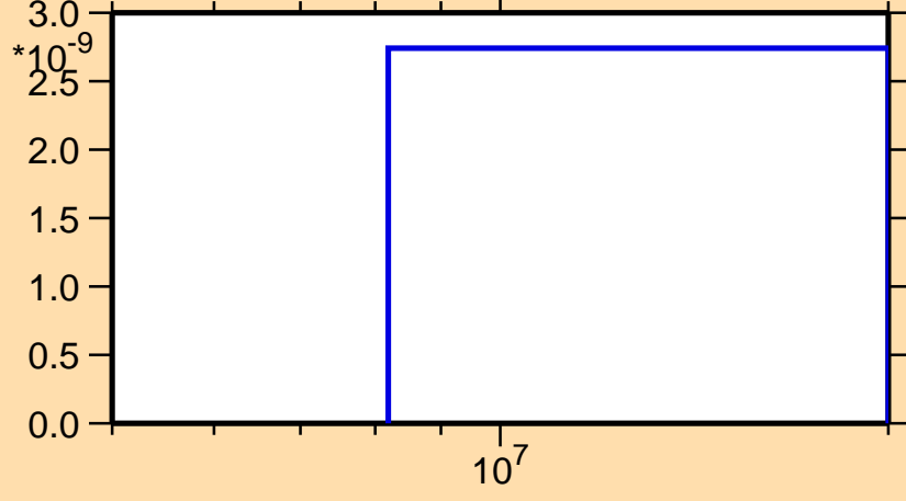
\sigma vs. E for ^{172}\text{Ho}(n,2np)
