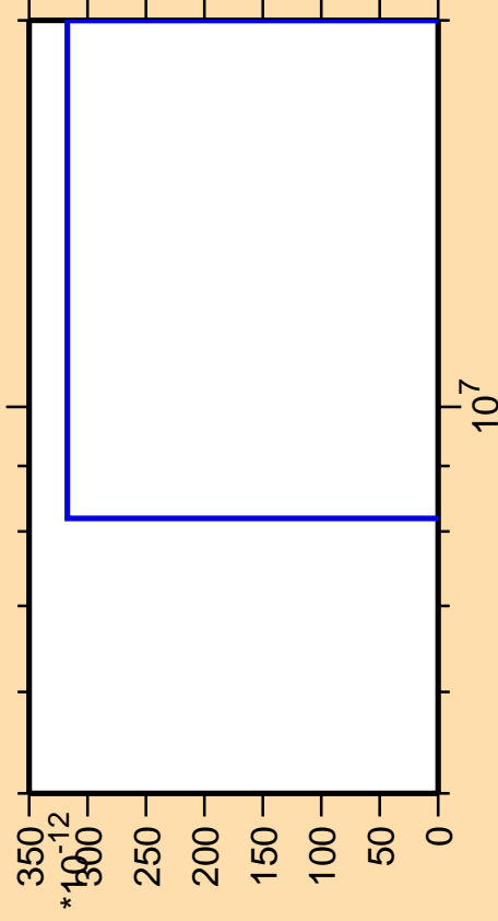
\Delta\sigma/\sigma vs. E for ^{172}\text{Ho} (mt 42)
