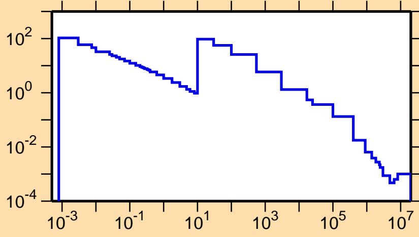
\sigma vs. E for ^{172}\text{Ho}(n,\gamma)
