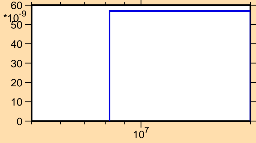
\sigma vs. E for ^{172}\text{Ho}(n,nt)
