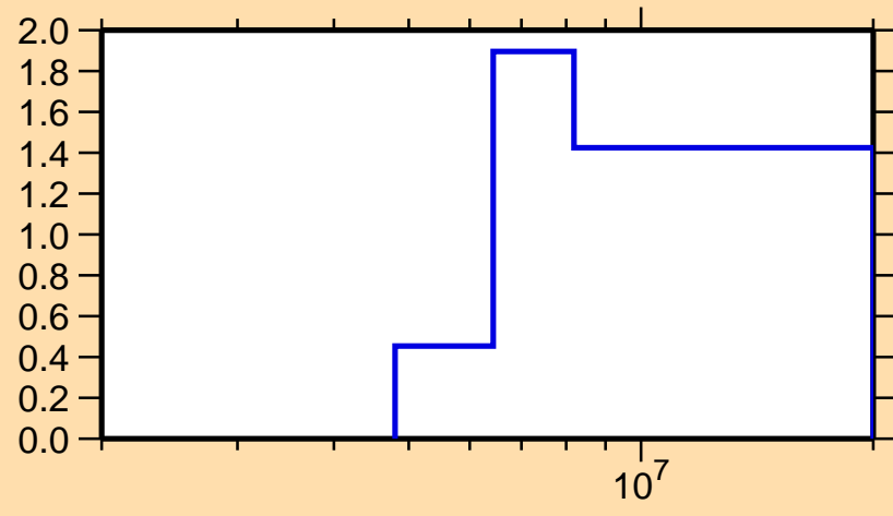
\sigma vs. E for ^{172}\text{Ho}(n,2n)
