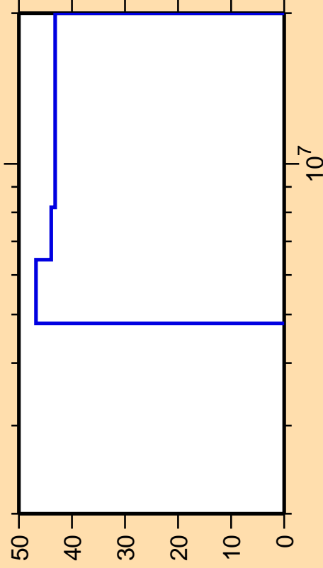
\Delta\sigma/\sigma vs. E for ^{172}\text{Ho}(n,n\text{cont.})
