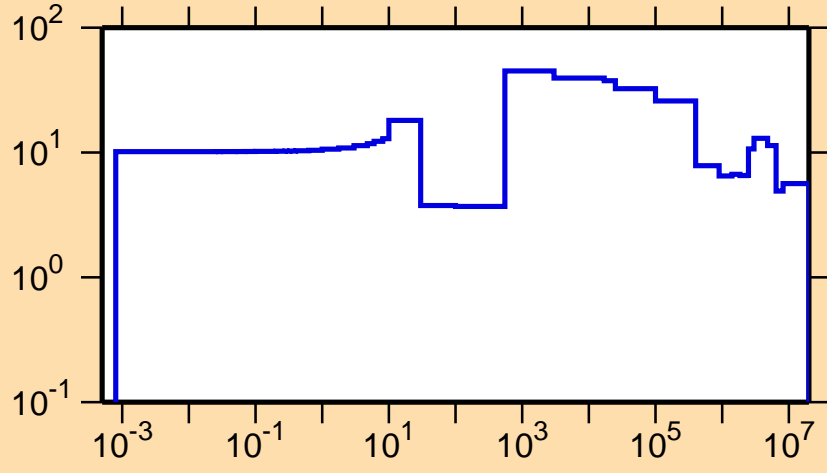
\Delta\sigma/\sigma vs. E for ^{172}\text{Ho}(n,\text{el.})
