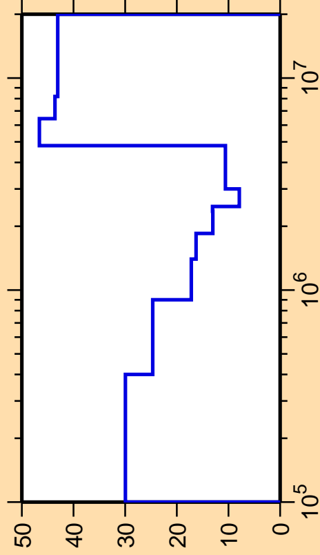
\Delta\sigma/\sigma vs. E for ^{172}\text{Ho}(n,\text{inel.})
