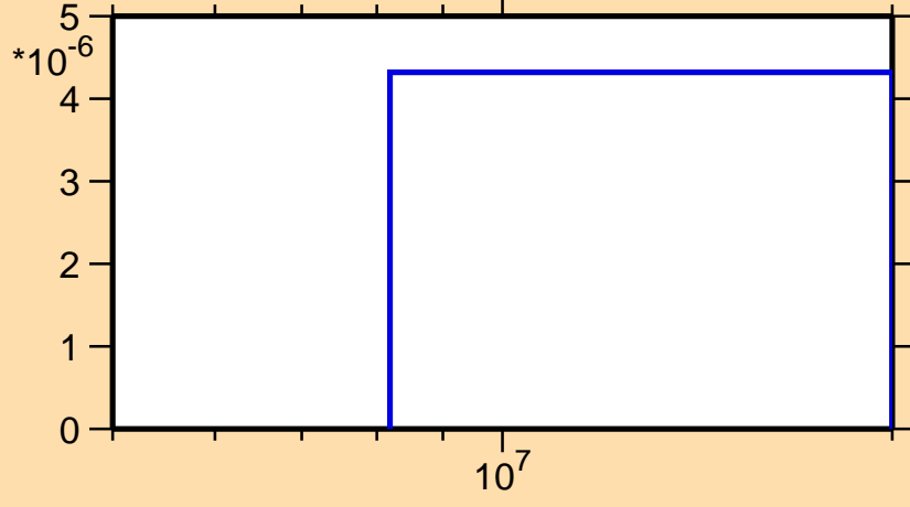
\sigma vs. E for ^{172}\text{Ho}(n,n\alpha)
