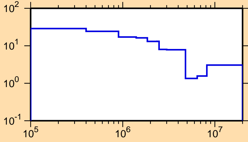
\Delta\sigma/\sigma vs. E for ^{172}\text{Ho}(n,n\text{onel.})
