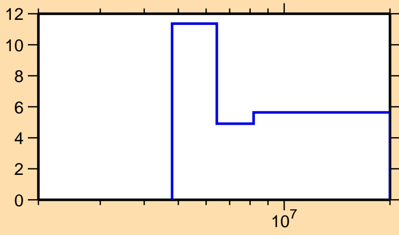
\Delta\sigma/\sigma vs. E for ^{172}\text{Ho}(n,\text{el.})
