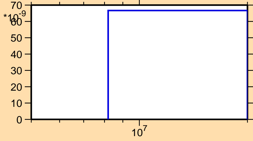
\sigma vs. E for ^{172}\text{Ho}(n,\text{nd})
