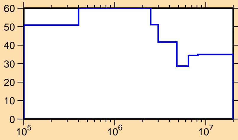
\Delta\sigma/\sigma vs. E for ^{172}\text{Ho}(n,n_1)
