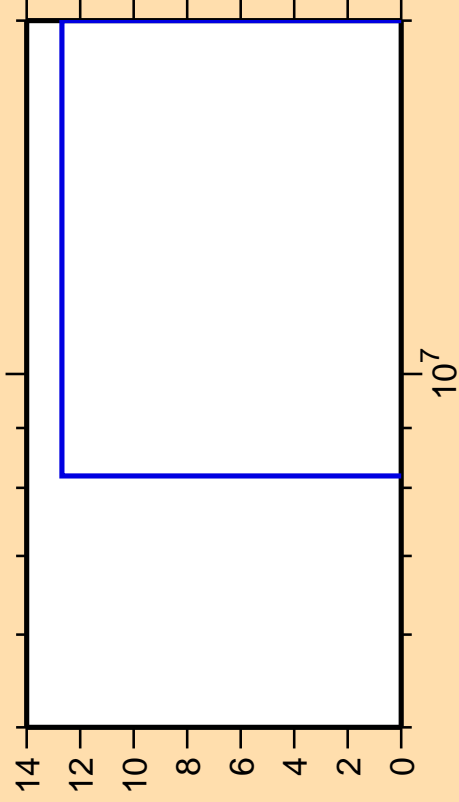
\Delta\sigma/\sigma vs. E for ^{172}\text{Ho}(n,3n)
