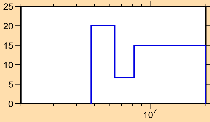
\Delta\sigma/\sigma vs. E for ^{172}\text{Ho}(n,2n)
