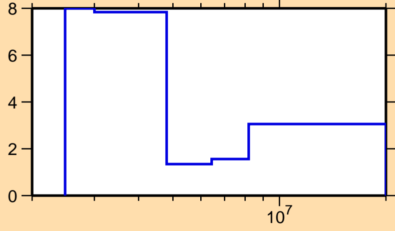
\Delta\sigma/\sigma vs. E for ^{172}\text{Ho}(n,\text{nonel.})
