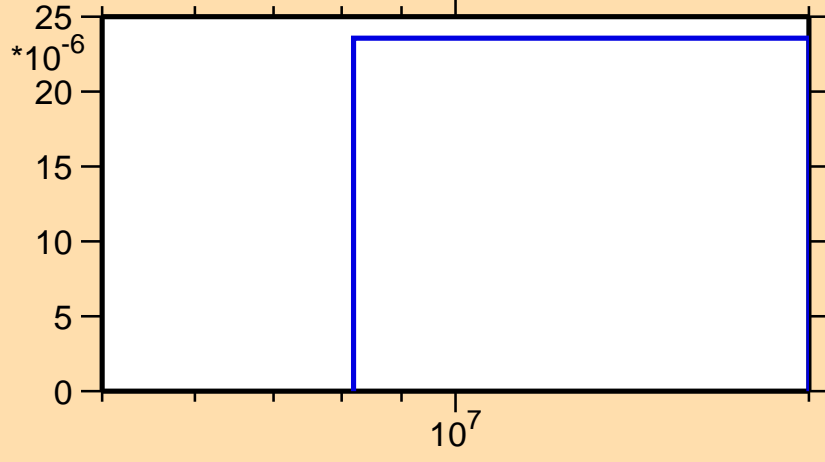
\sigma vs. E for ^{172}\text{Ho}(n,t)
