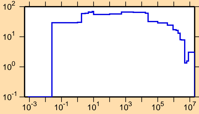
\Delta\sigma/\sigma vs. E for ^{172}\text{Ho}(n,\text{nonel.})
