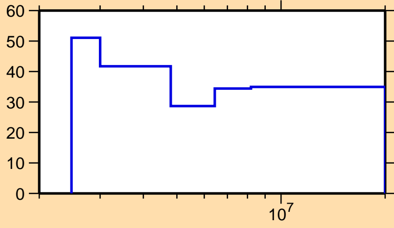
\Delta\sigma/\sigma vs. E for ^{172}\text{Ho}(n,n_1)
