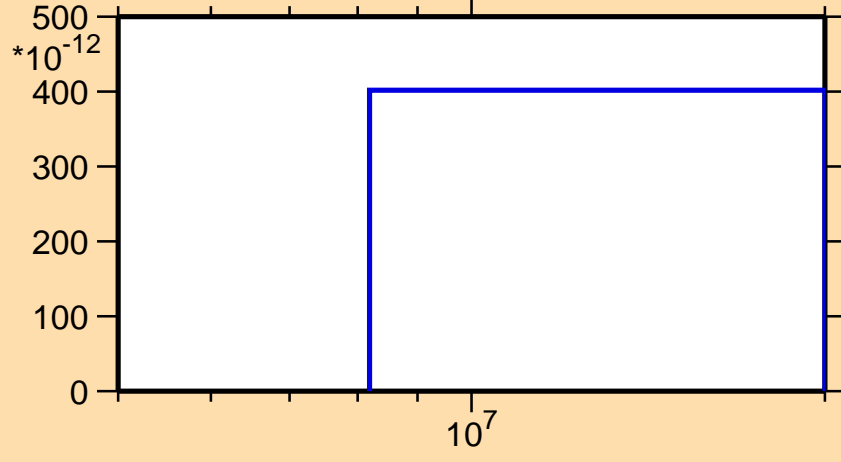
\sigma vs. E for ^{172}\text{Ho}(n,2n\alpha)
