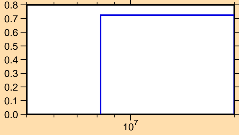
\sigma vs. E for ^{172}\text{Ho}(n,3n)
