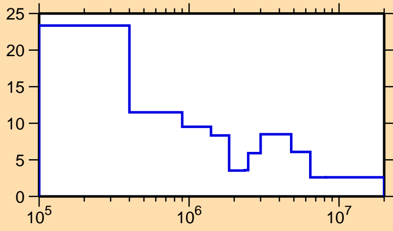
\Delta\sigma/\sigma vs. E for ^{172}\text{Ho}(n,\text{tot.})
