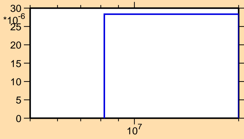
\sigma vs. E for ^{172}\text{Ho}(n,np)
