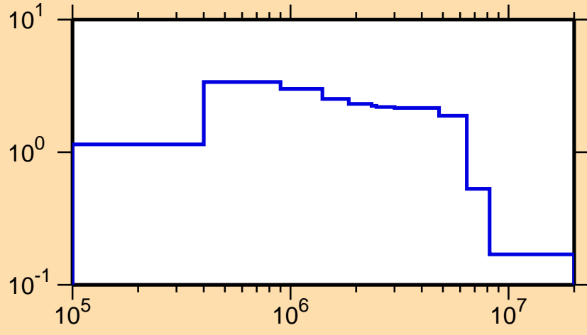
\sigma vs. E for ^{172}\text{Ho}(n,\text{inel.})
