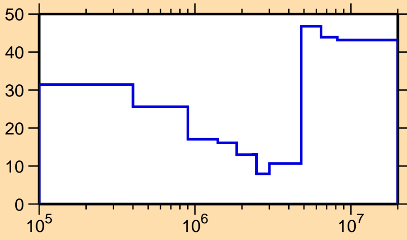
\Delta\sigma/\sigma vs. E for ^{172}\text{Ho}(n,n\text{cont.})
