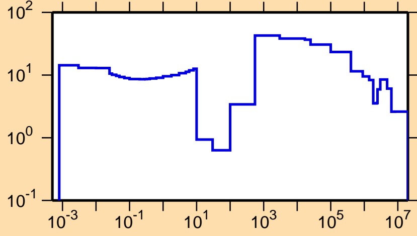
\Delta\sigma/\sigma vs. E for ^{172}\text{Ho}(n,\text{tot.})
