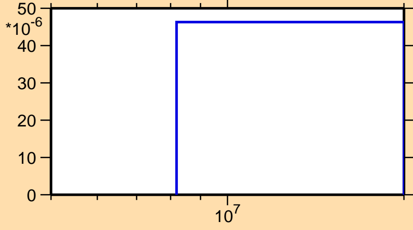
\sigma vs. E for ^{172}\text{Ho}(n,d)
