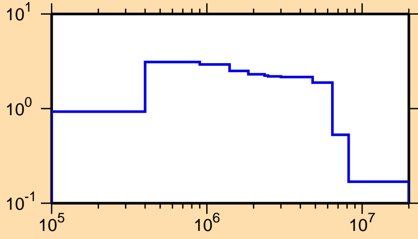
\sigma vs. E for ^{172}\text{Ho}(n,n\text{cont.})
