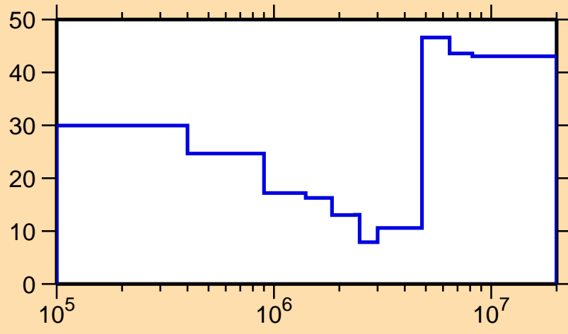
\Delta\sigma/\sigma vs. E for ^{172}\text{Ho}(n,\text{inel.})
