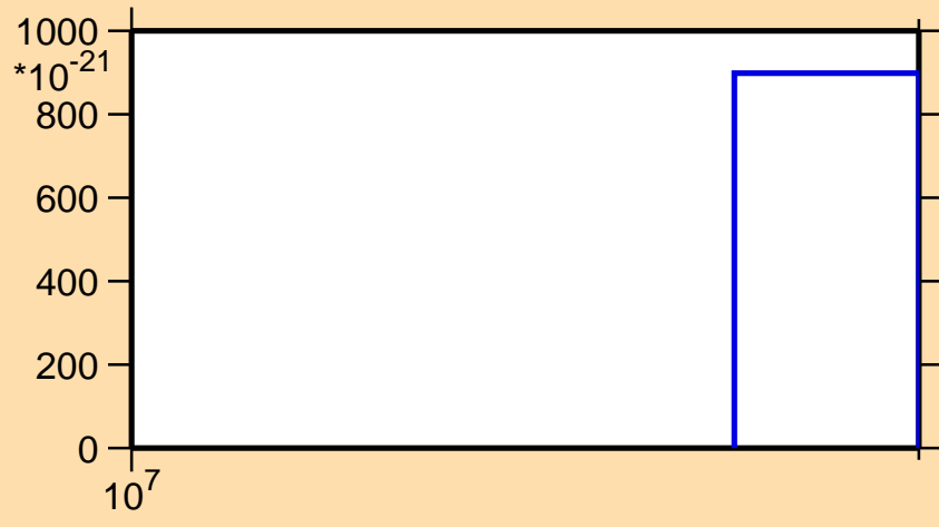
\sigma vs. E for ^{173}\text{Ho} (mt 42)
