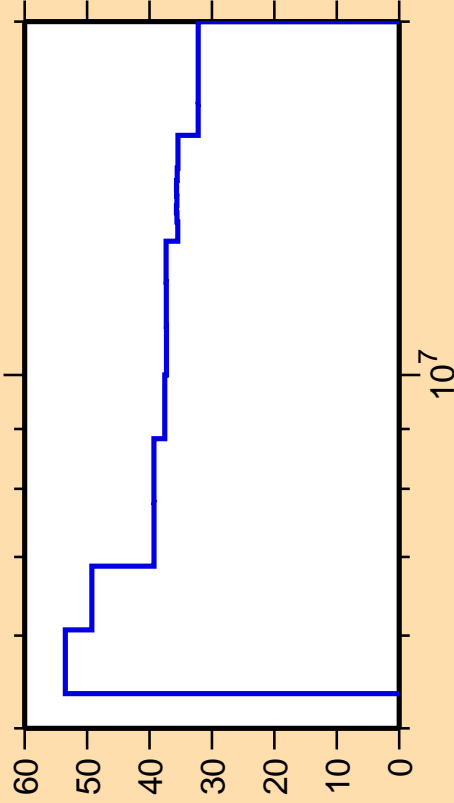
\Delta\sigma/\sigma vs. E for ^{173}\text{Ho}(n,n_1)
