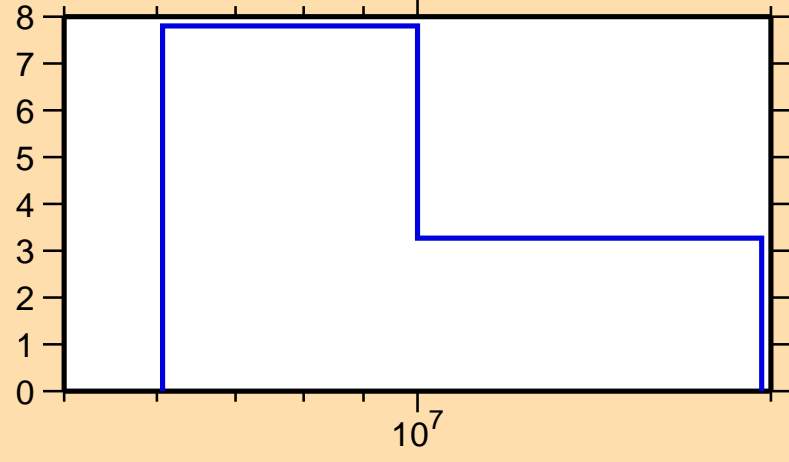
\Delta\sigma/\sigma vs. E for ^{173}\text{Ho}(n,el.)
