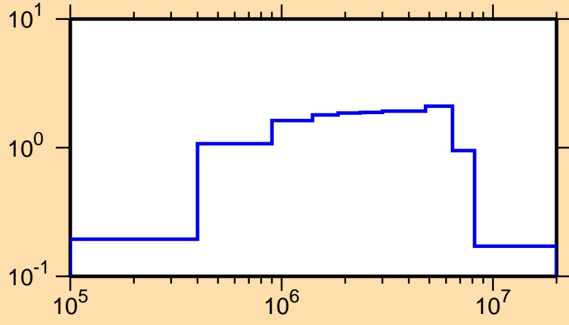
\sigma vs. E for ^{173}\text{Ho}(n,n\text{cont.})
