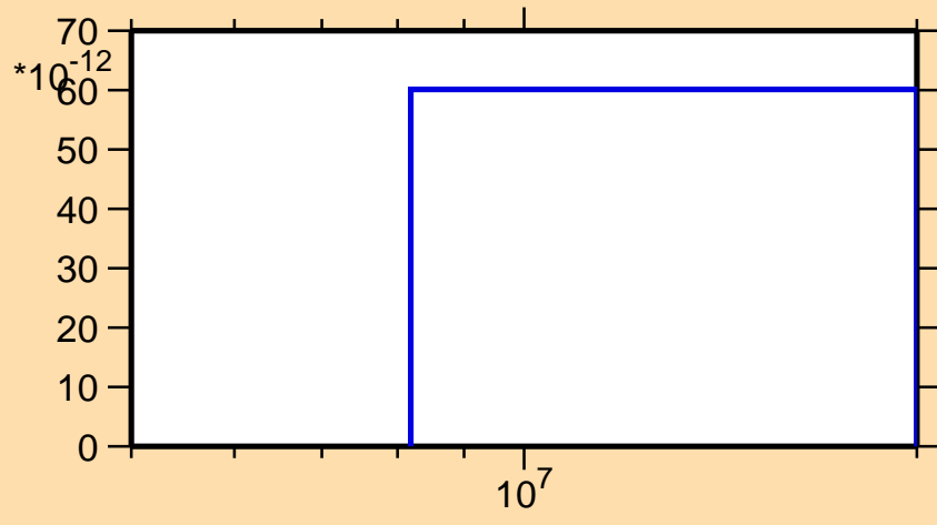
\sigma vs. E for ^{173}\text{Ho}(n,2n\alpha)
