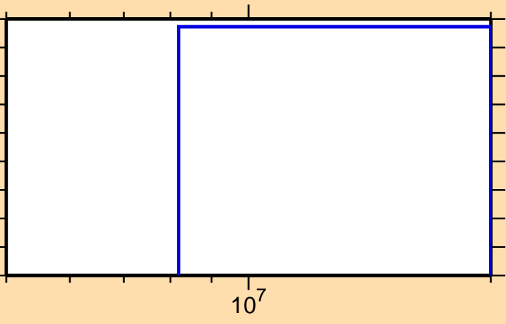
\sigma vs. E for ^{173}\text{Ho}(n,np)
