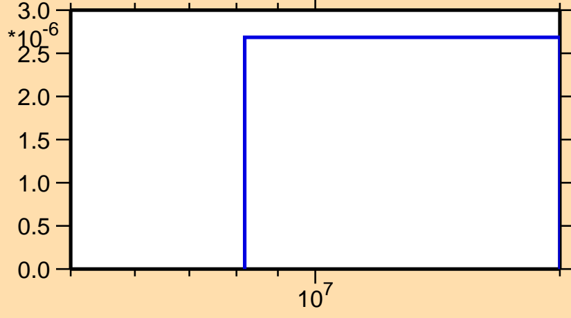
\sigma vs. E for ^{173}\text{Ho}(n,n\alpha)
