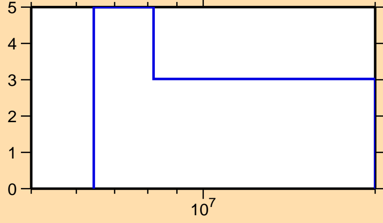
\Delta\sigma/\sigma vs. E for ^{173}\text{Ho}(n,\text{tot.})
