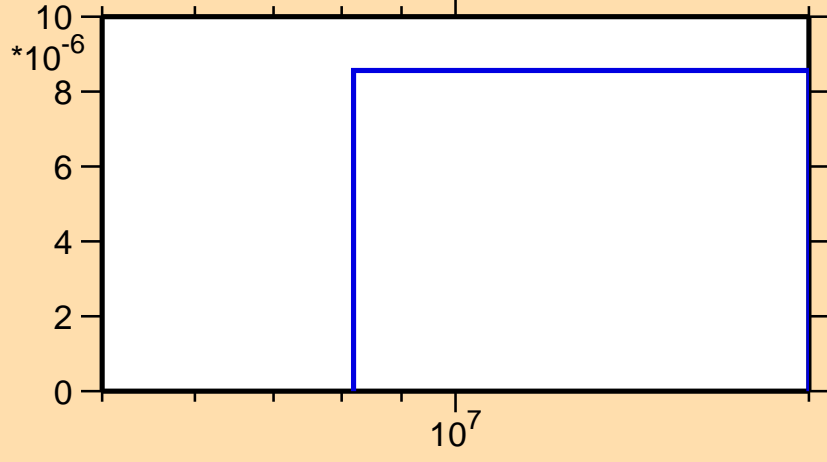
\sigma vs. E for ^{173}\text{Ho}(n,t)
