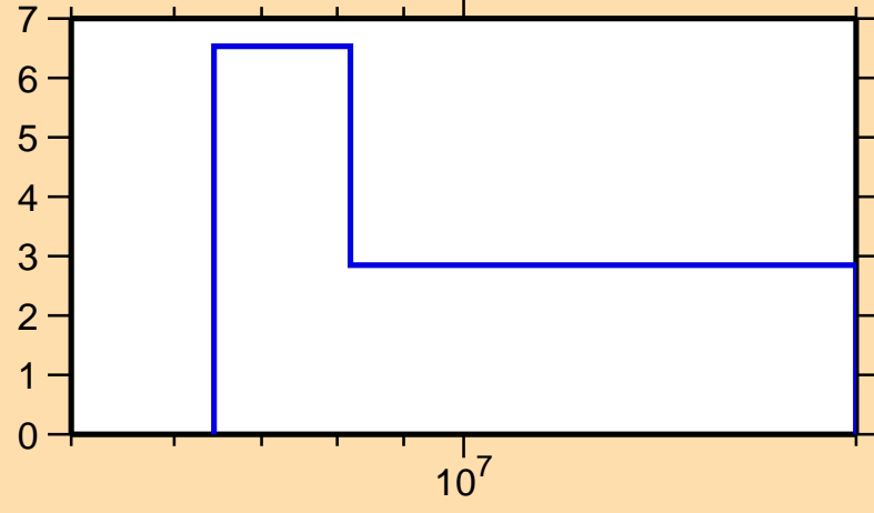
\Delta\sigma/\sigma vs. E for ^{173}\text{Ho}(n,\text{el.})
