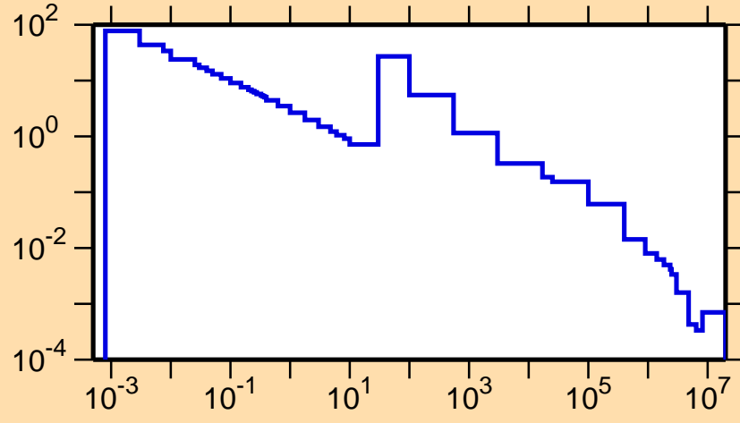
\sigma vs. E for ^{173}\text{Ho}(n,\gamma)
