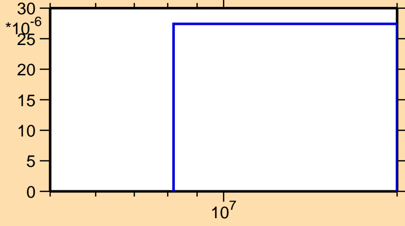
\sigma vs. E for ^{173}\text{Ho}(n,d)
