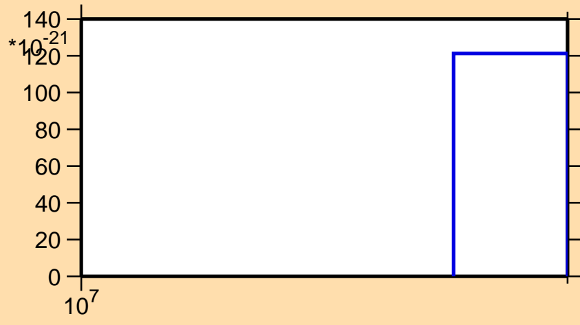
\sigma vs. E for ^{174}\text{Ho} (mt 42)
