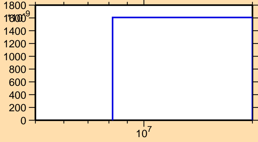
\sigma vs. E for ^{174}\text{Ho}(n,n\alpha)
