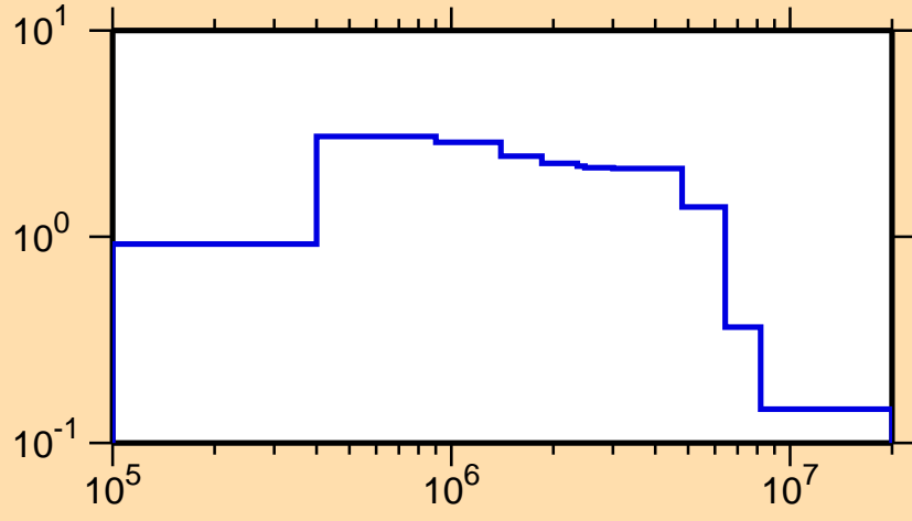
\sigma vs. E for ^{174}\text{Ho}(n,n\text{cont.})
