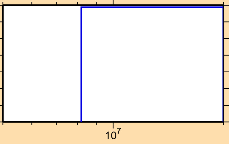
\sigma vs. E for ^{174}\text{Ho}(n,t)
