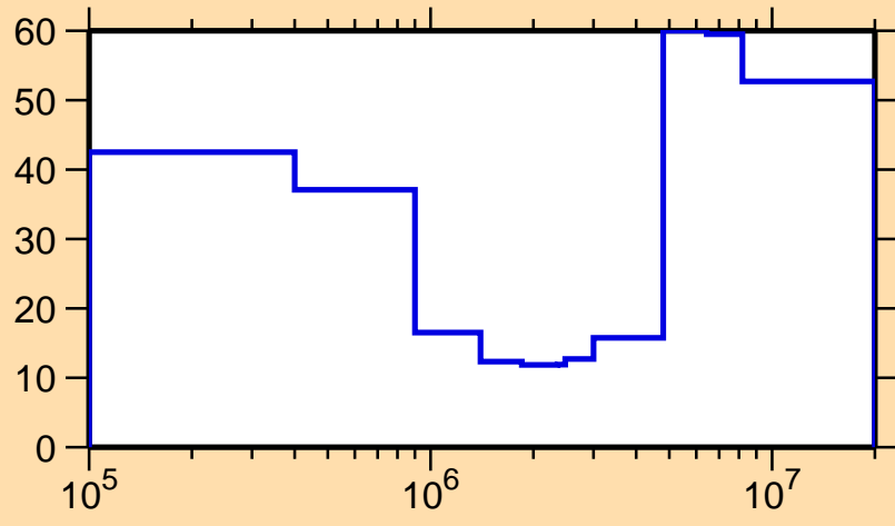
\Delta\sigma/\sigma vs. E for ^{174}\text{Ho}(n,n\text{cont.})
