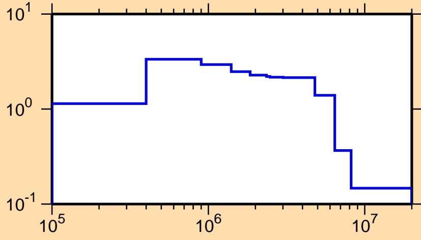
\sigma vs. E for ^{174}\text{Ho}(n,\text{inel.})
