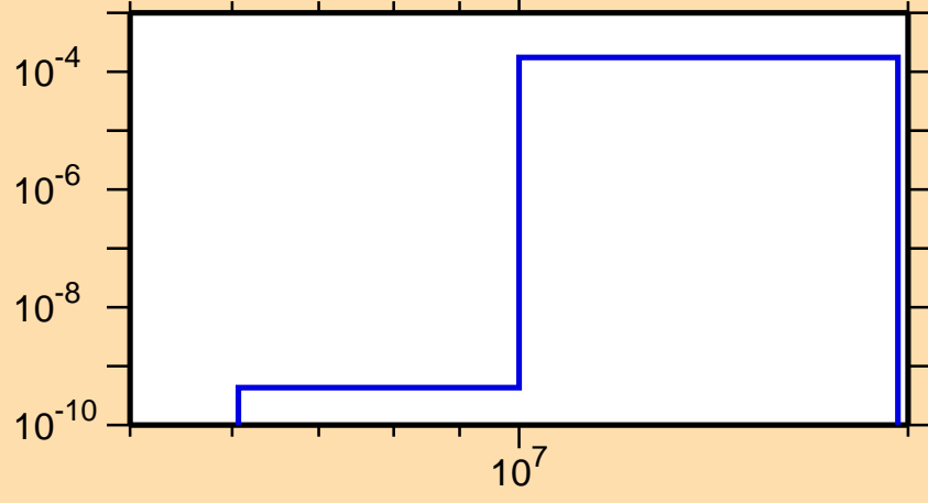
\sigma vs. E for ^{175}\text{Ho}(n,p)
