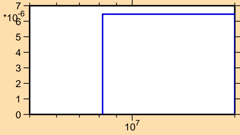
\sigma vs. E for ^{175}\text{Ho}(n,np)
