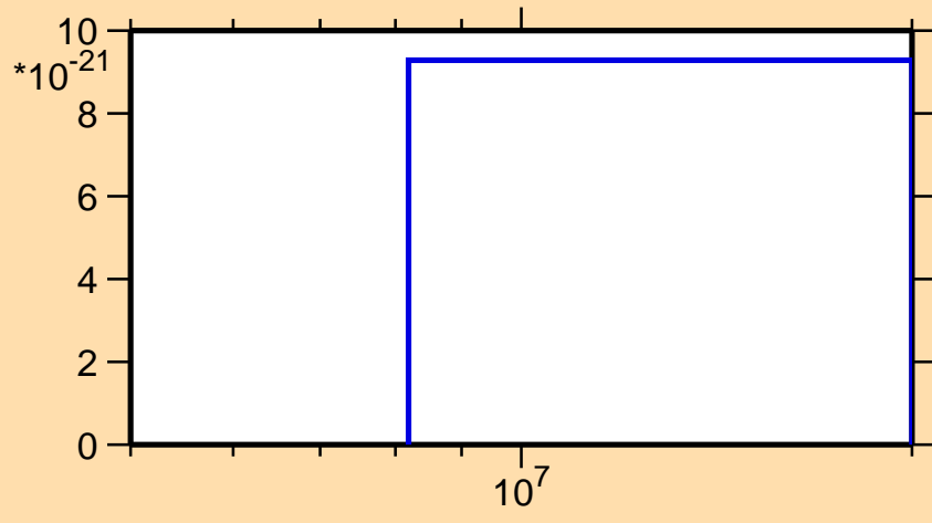
\sigma vs. E for ^{175}\text{Ho} (mt 42)
