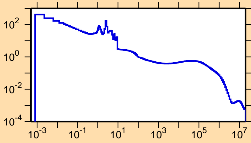
\sigma vs. E for ^{269}\gamma
