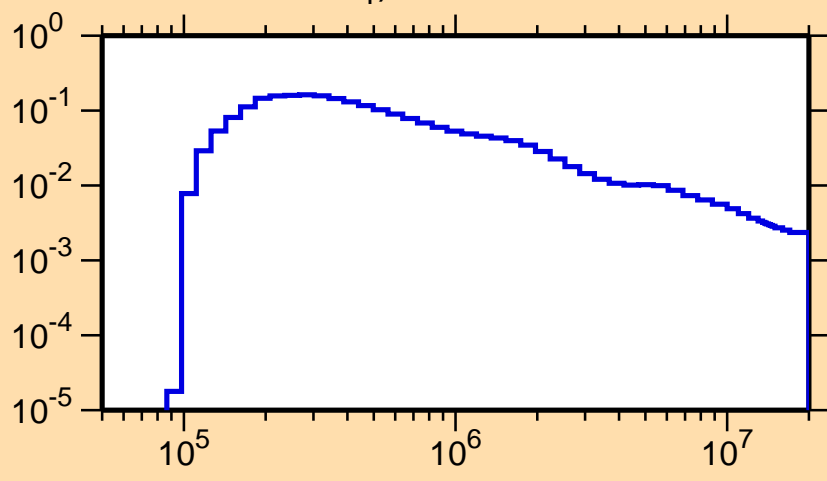
\sigma vs. E for ^{270}_{1}
