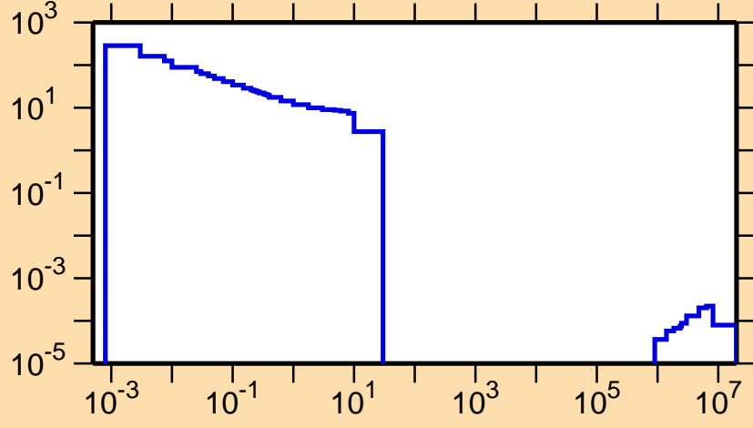
\sigma vs. E for ^{271}\gamma
