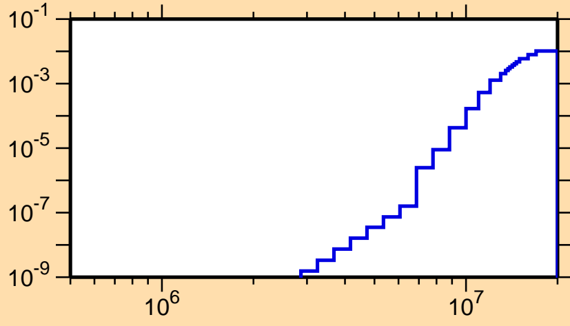
\sigma vs. E for ^{111}\text{I}(n,\text{He3})
