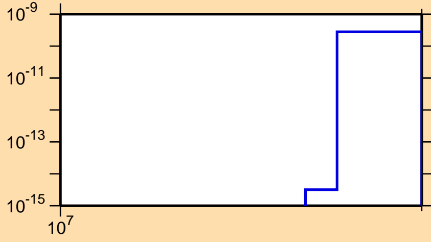
\sigma vs. E for ^{111}\text{I}(n,nt)
