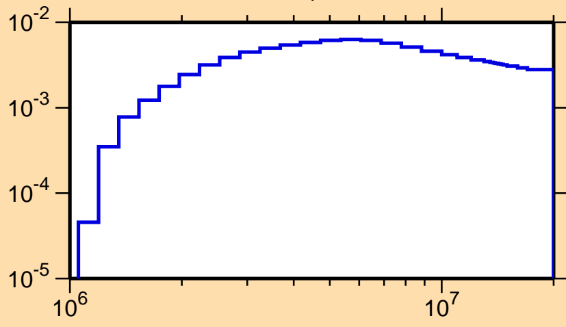
\sigma vs. E for ^{111}\text{I}(n,n_4)
