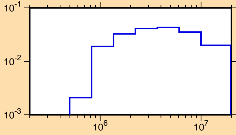
\sigma vs. E for ^{111}\text{I}(n,n_2)
