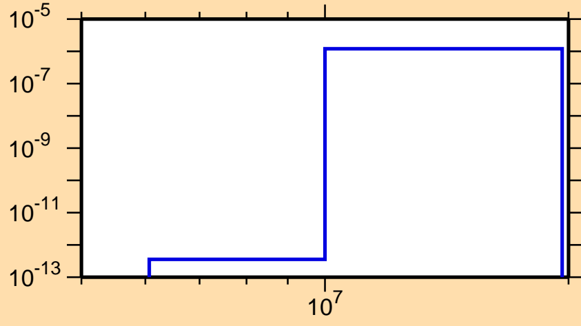
\sigma vs. E for ^{111}\text{I}(n,2n\alpha)
