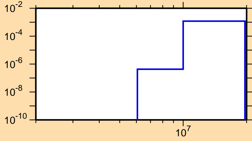
\sigma vs. E for ^{111}\text{I} (mt 45)
