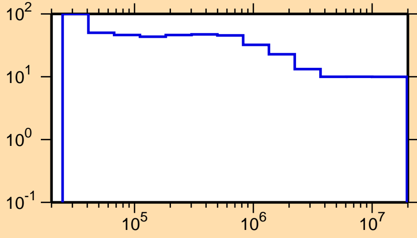
\Delta\sigma/\sigma vs. E for ^{111}\text{I}(n,\text{nonel.})
