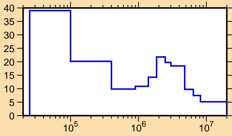
\Delta\sigma/\sigma vs. E for ^{111}\text{I}(n,\text{tot.})
