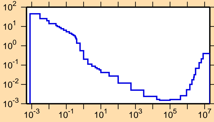
\sigma vs. E for ^{111}\text{I}(n,p\alpha)
