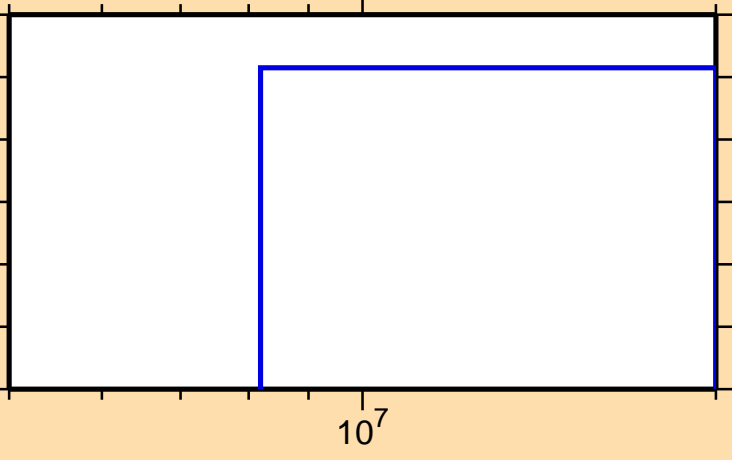
\sigma vs. E for ^{111}\text{I}(n,2n)
