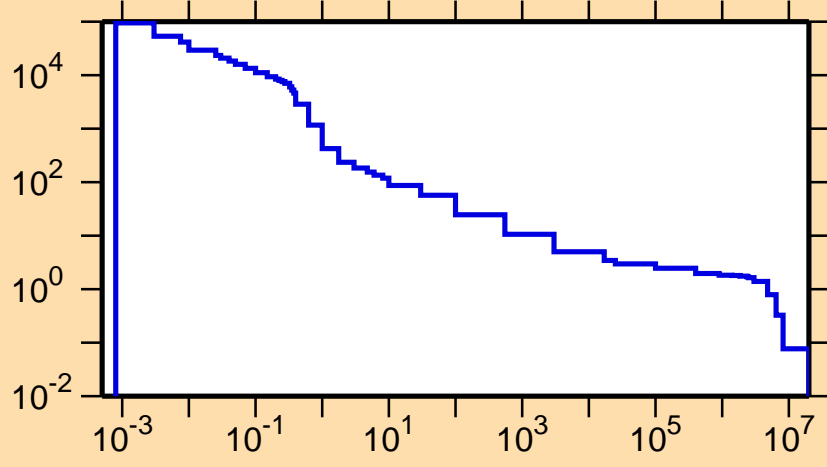
\sigma vs. E for ^{111}\text{I}(n,p)
