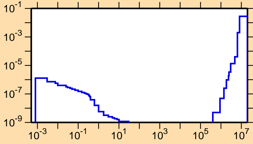
\sigma vs. E for ^{111}\text{I}(n,d)
