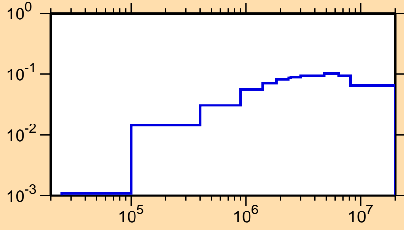
\sigma vs. E for ^{111}\text{I}(n,\text{inel.})
