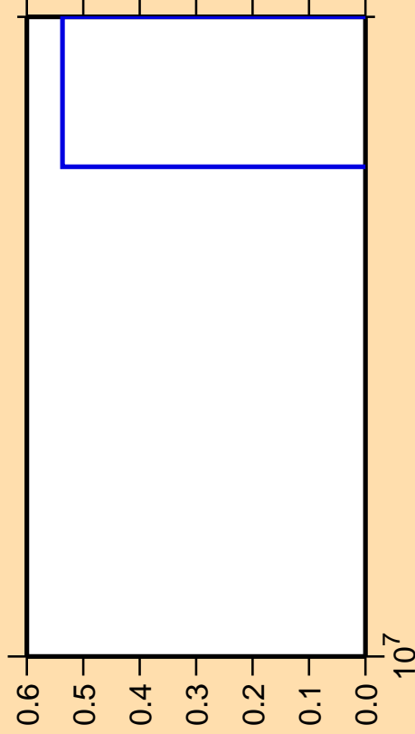
\Delta\sigma/\sigma vs. E for ^{112}\text{I}(n,3n\alpha)
