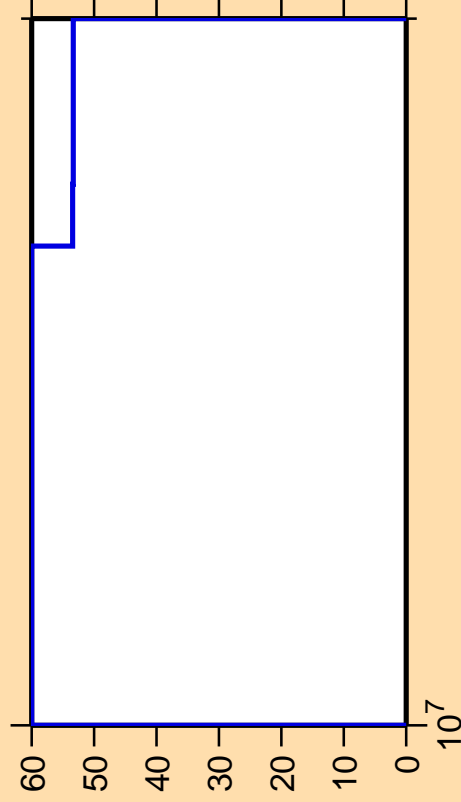
\Delta\sigma/\sigma vs. E for ^{112}\text{I}(n,\gamma)
