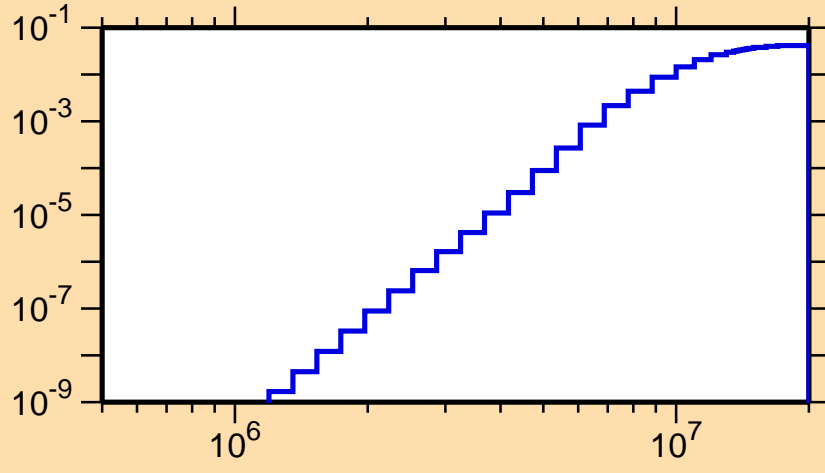
\sigma vs. E for ^{112}\text{I}(n,d)
