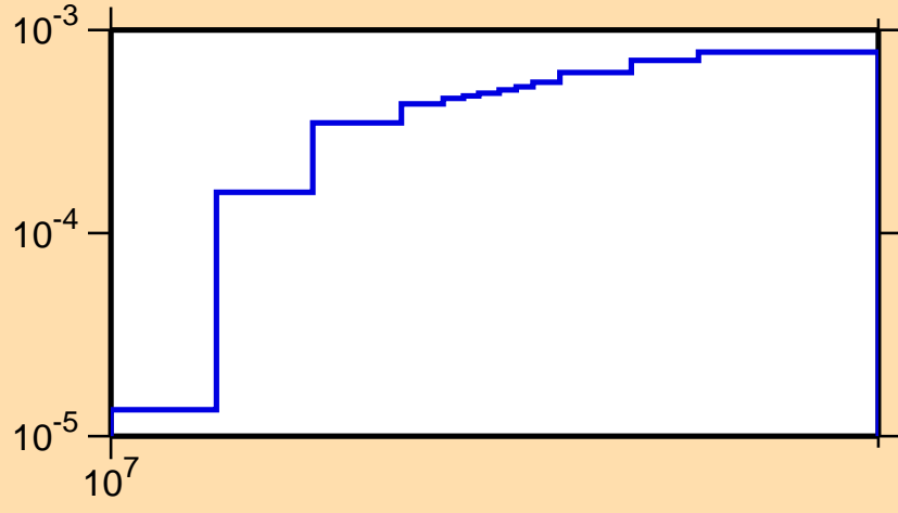
\sigma vs. E for ^{112}\text{I}(n,2n)
