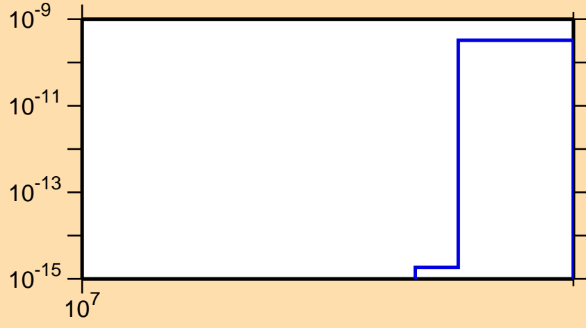
\sigma vs. E for ^{112}\text{I}(n,nt)
