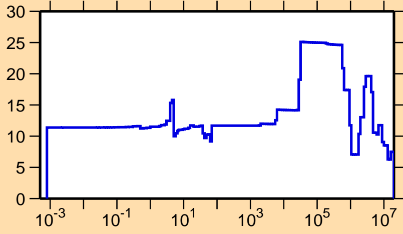
\Delta\sigma/\sigma vs. E for ^{112}\text{I}(n,\text{el.})
