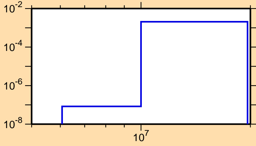
\sigma vs. E for ^{112}\text{I}(n,\text{pd})
