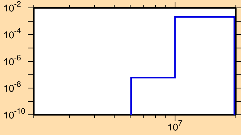
\sigma vs. E for ^{112}\text{I}(\text{mt } 45)
