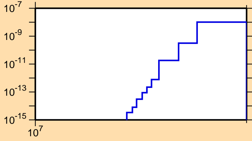
\sigma vs. E for ^{113}\text{I} (mt 34)
