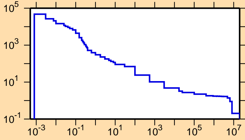
\sigma vs. E for ^{114}\text{I}(n,p)
