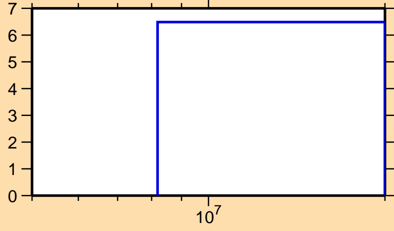
\Delta\sigma/\sigma vs. E for ^{114}\text{I}(n,\text{el.})
