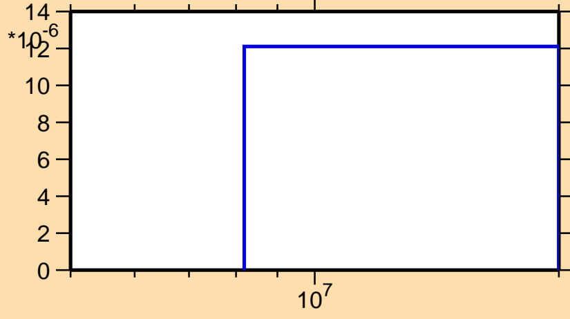
\sigma vs. E for ^{114}\text{I}(n,\text{pt})
