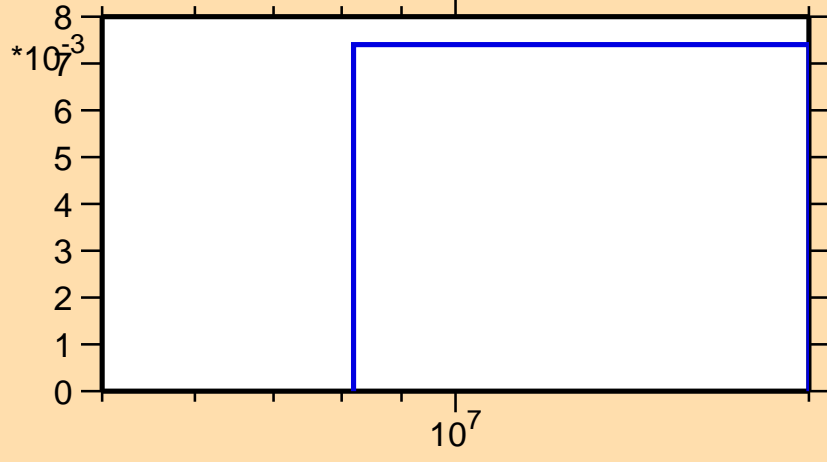
\sigma vs. E for ^{114}\text{I}(n,2n)
