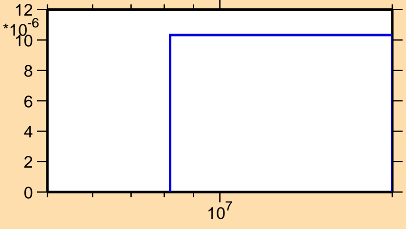
\sigma vs. E for ^{114}\text{I}(n,\text{nd})
