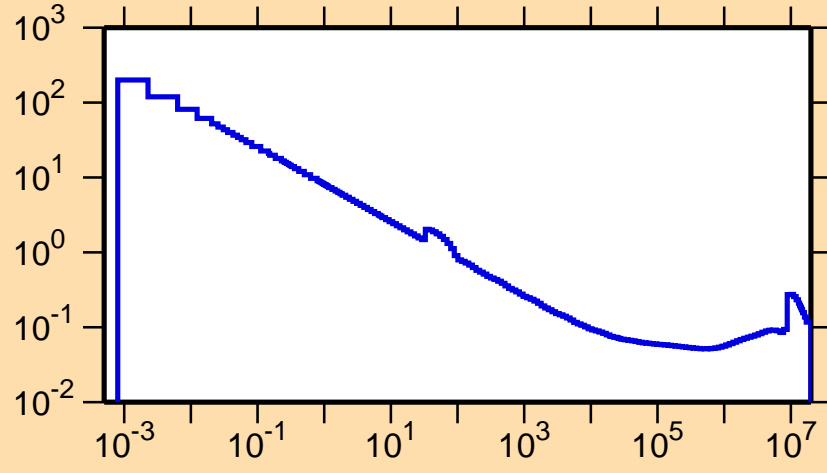
\sigma vs. E for ^{114}\text{I}(n,\alpha)
