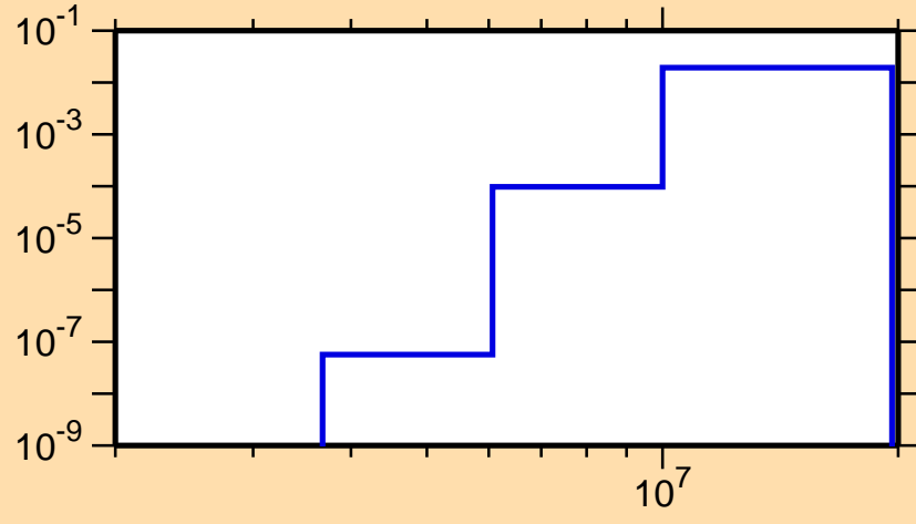
\sigma vs. E for ^{114}\text{I}(n,n\alpha)
