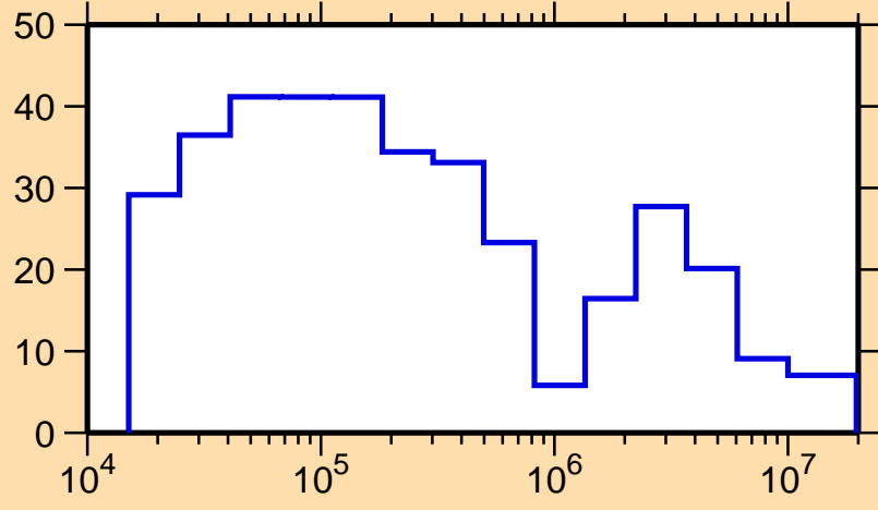
\Delta\sigma/\sigma vs. E for ^{114}\text{I}(n, el.)
