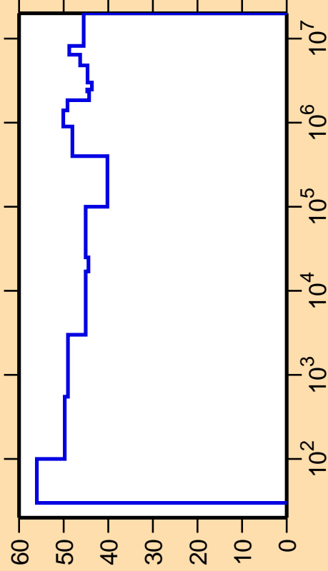
\Delta\sigma/\sigma vs. E for ^{114}\text{I}(n,\text{inel.})
