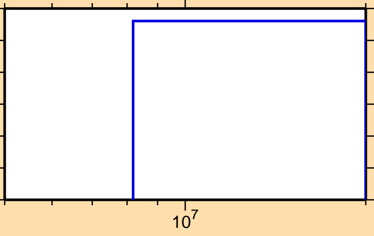
\sigma vs. E for ^{114}\text{I}(n,2n\alpha)
