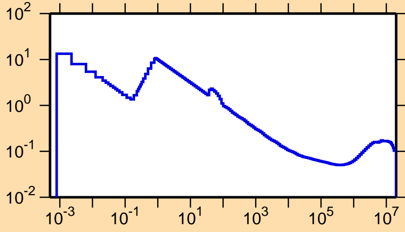
\sigma vs. E for ^{115}\text{I}(n,\alpha)
