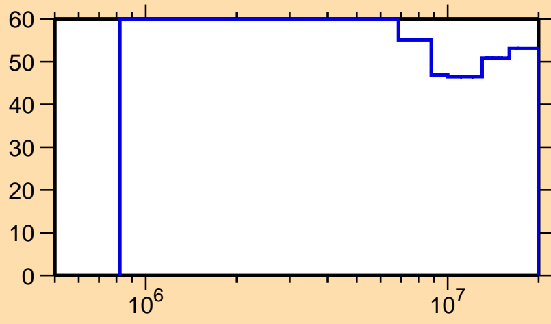
\Delta\sigma/\sigma vs. E for ^{115}\text{I}(n,n\text{cont.})
