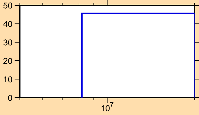
\Delta\sigma/\sigma vs. E for ^{115}\text{I}(n,\text{inel.})
