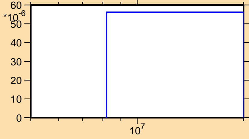
\sigma vs. E for ^{115}\text{I}(n,\text{pd})
