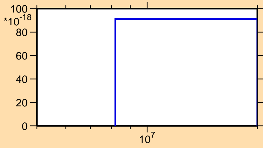
\sigma vs. E for ^{115}\text{I}(n,3n\alpha)
