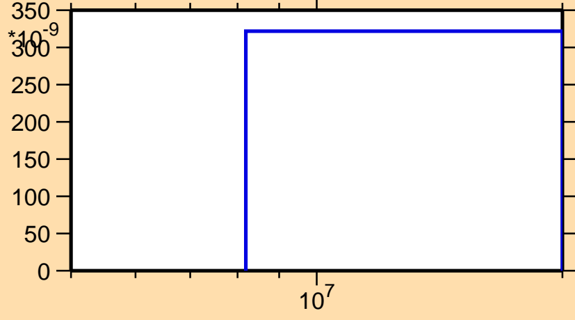
\sigma vs. E for ^{115}\text{I}(n,\text{nd})
