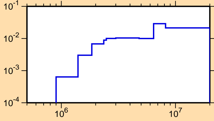
\sigma vs. E for ^{115}\text{I}(n,n\text{cont.})
