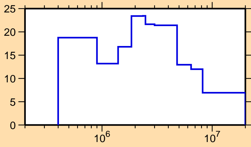
\Delta\sigma/\sigma vs. E for ^{115}\text{I}(n,\text{el.})
