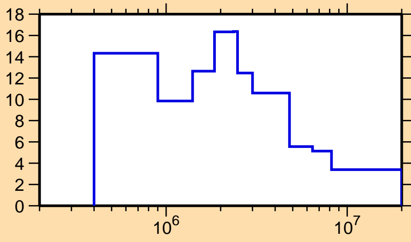
\Delta\sigma/\sigma vs. E for ^{115}\text{I}(n,\text{tot.})
