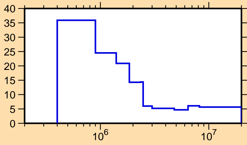
\Delta\sigma/\sigma vs. E for ^{115}\text{I}(n, nonel.)
