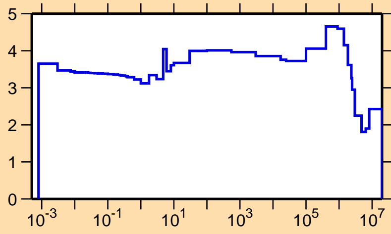
\sigma vs. E for ^{115}\text{I}(n,\text{el.})
