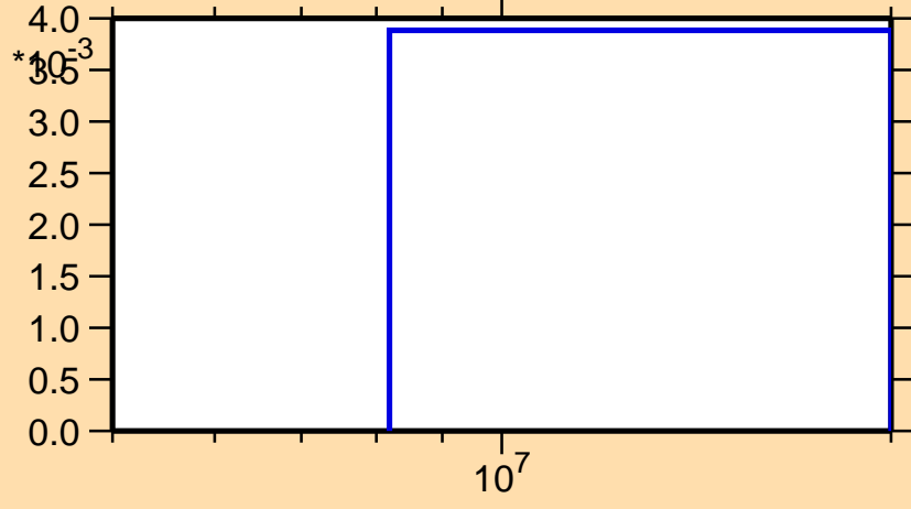
\sigma vs. E for ^{115}\text{I}(n,2n)
