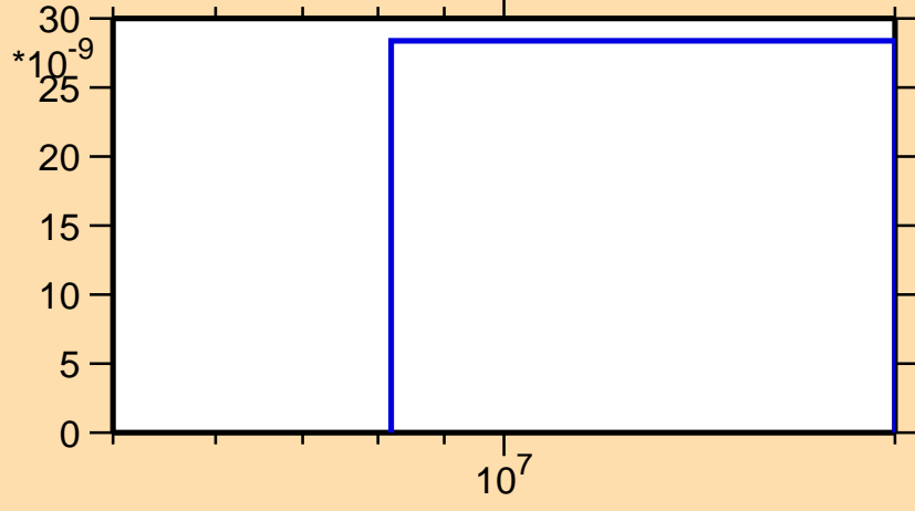
\sigma vs. E for ^{115}\text{I}(n,\text{pt})
