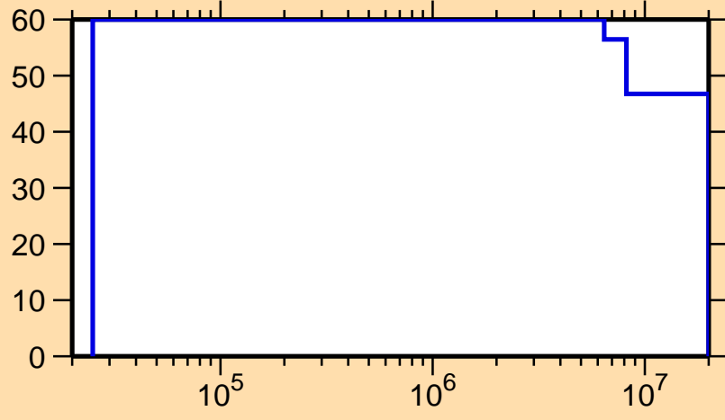
\Delta\sigma/\sigma vs. E for ^{115}\text{I}(n,n_1)
