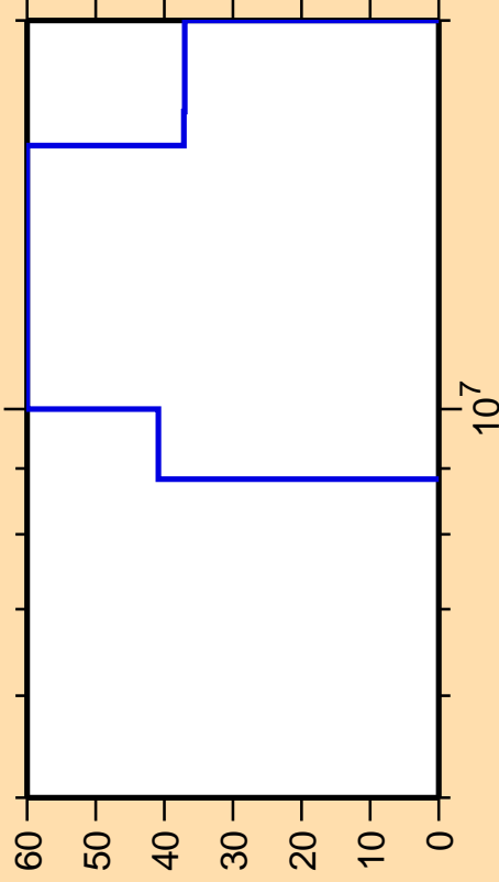
\Delta\sigma/\sigma vs. E for ^{116}\text{I}(\text{mt } 45)
