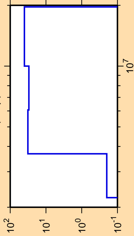
\Delta\sigma/\sigma vs. E for ^{116}\text{I}(n,np)
