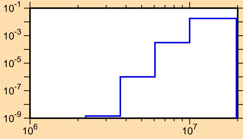
\sigma vs. E for ^{116}\text{I}(n,d)
