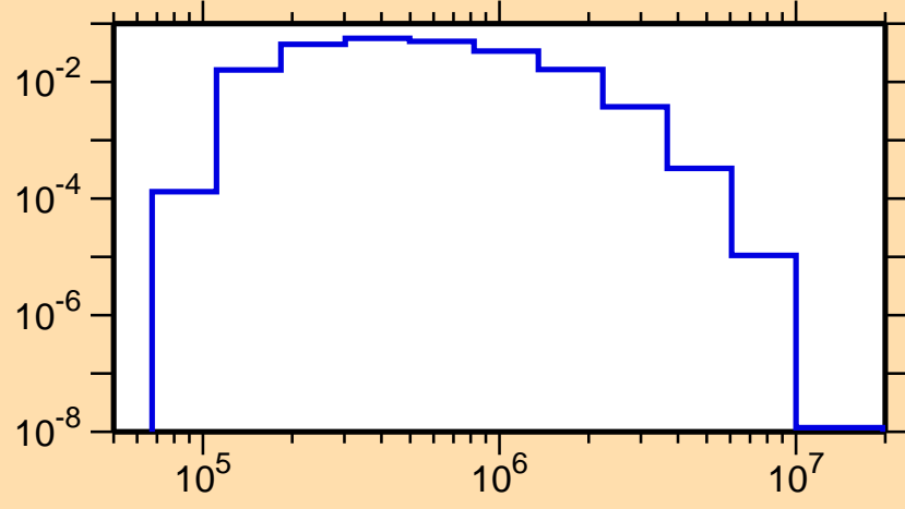
\sigma vs. E for ^{116}\text{I}(n,n_1)
