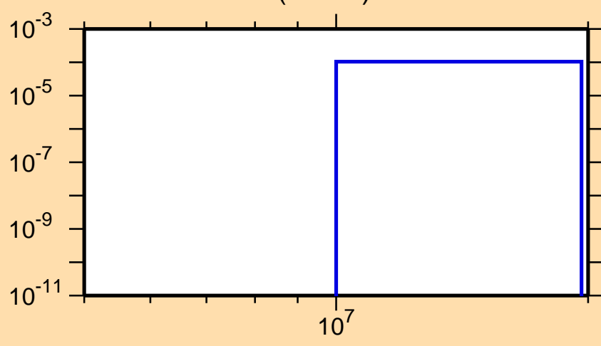
\sigma vs. E for ^{116}\text{I}(\text{mt } 45)
