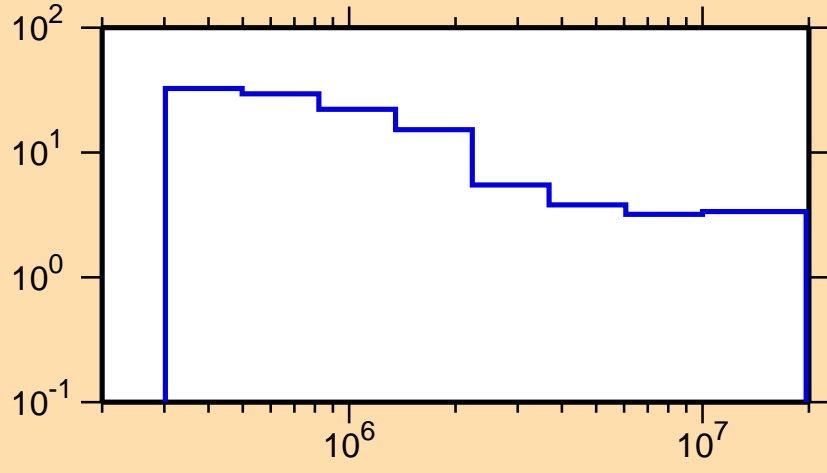
\Delta\sigma/\sigma vs. E for ^{116}\text{I}(n, nonel.)
