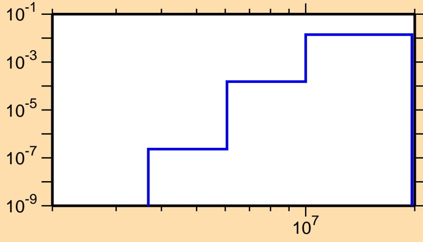
\sigma vs. E for ^{118}\text{I}(n,d)
