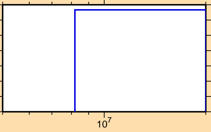
\sigma vs. E for ^{118}\text{I}(n,\text{nd})
