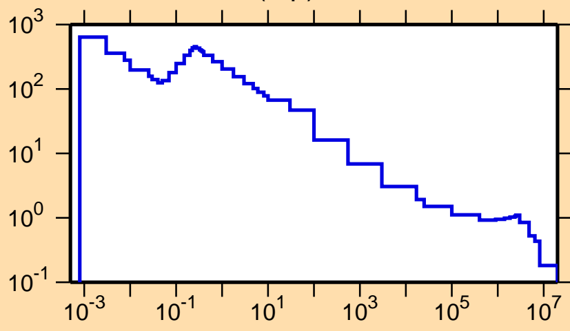
\sigma vs. E for ^{118}\text{I}(n,p)
