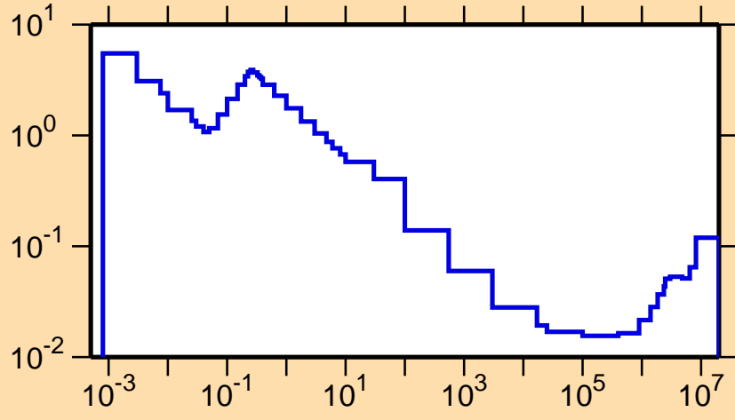
\sigma vs. E for ^{118}\text{I}(n,\alpha)
