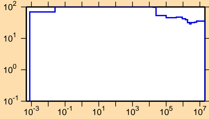
\Delta\sigma/\sigma vs. E for ^{118}\text{I}(n,p)
