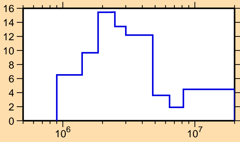
\Delta\sigma/\sigma vs. E for ^{118}\text{I}(n, tot.)
