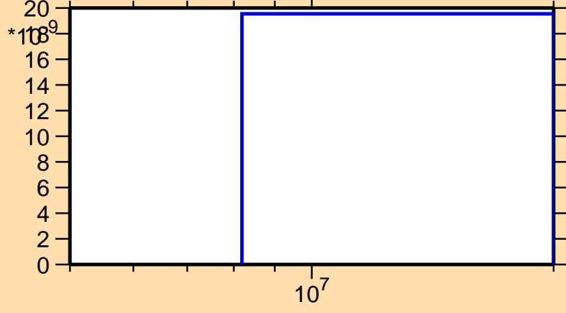
\sigma vs. E for ^{118}\text{I}(n,\text{pt})
