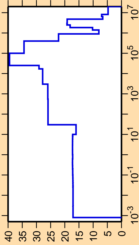
\Delta\sigma/\sigma vs. E for ^{118}\text{I}(n,\text{el.})
