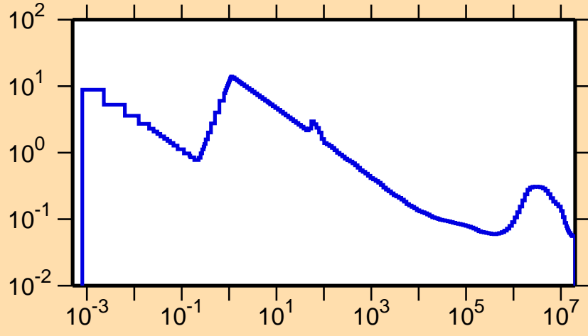
\sigma vs. E for ^{119}\text{I}(n,p)
