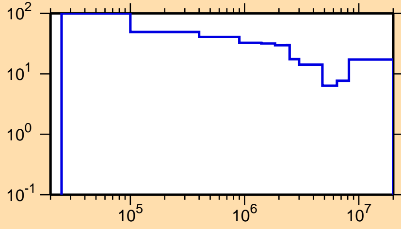
\Delta\sigma/\sigma vs. E for ^{119}\text{I}(n,\text{inel.})
