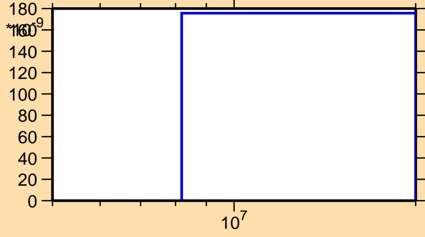
\sigma vs. E for ^{119}\text{I}(n,\text{nd})
