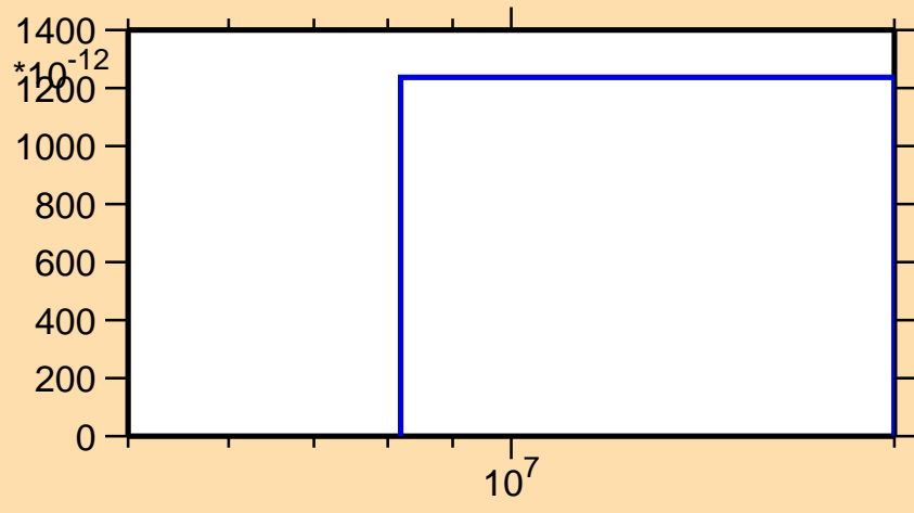
\sigma vs. E for ^{119}\text{I}(n,3n)
