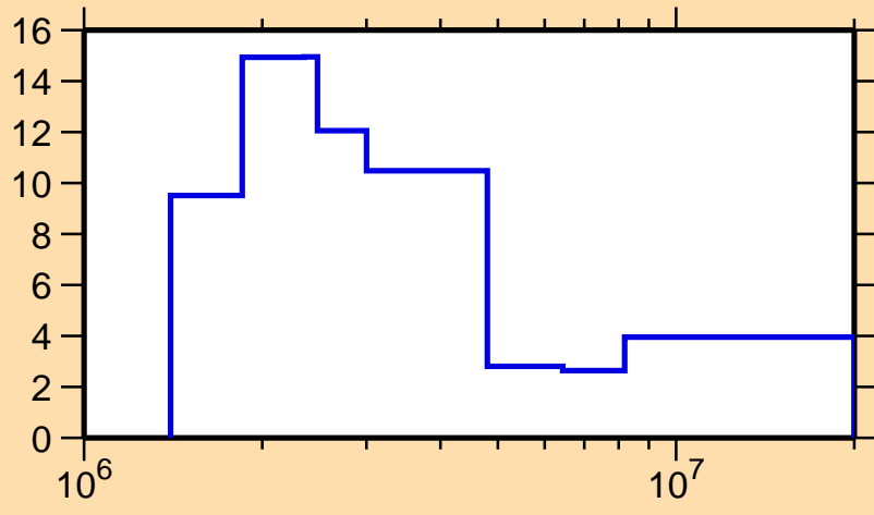
\Delta\sigma/\sigma vs. E for ^{119}\text{I}(n,\text{tot.})
