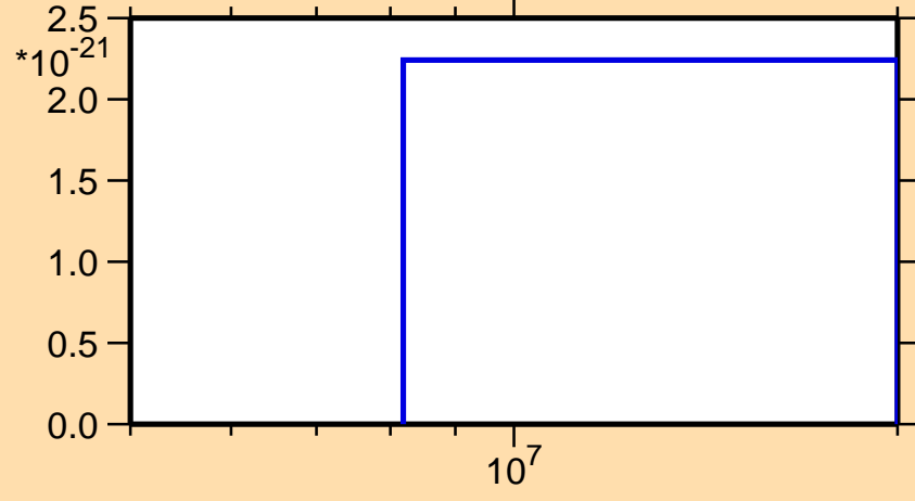
\sigma vs. E for ^{119}\text{I} (mt 11)
