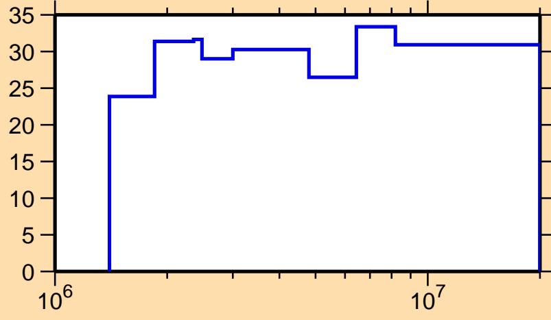
\Delta\sigma/\sigma vs. E for ^{119}\text{I}(n,n_1)
