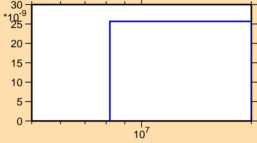
\sigma vs. E for ^{119}\text{I}(n,\text{pd})
