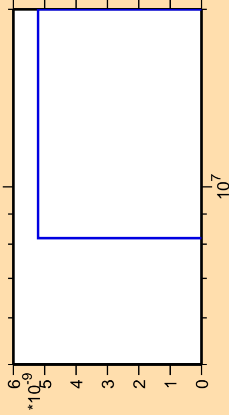
\Delta\sigma/\sigma vs. E for ^{119}\text{I} (mt 11)
