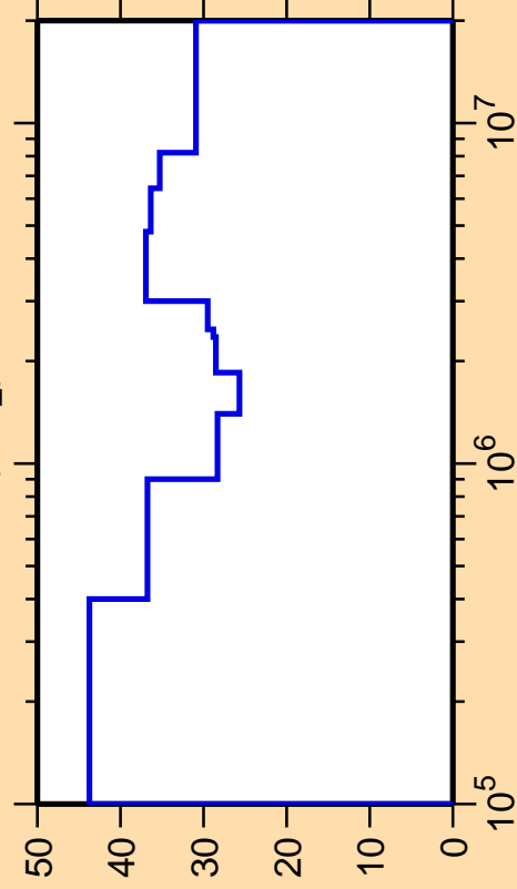
\Delta\sigma/\sigma vs. E for ^{119}\text{I}(n,n_2)
