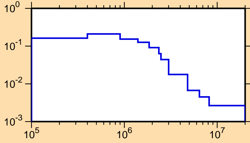
\sigma vs. E for ^{119}\text{I}(n,n_2)
