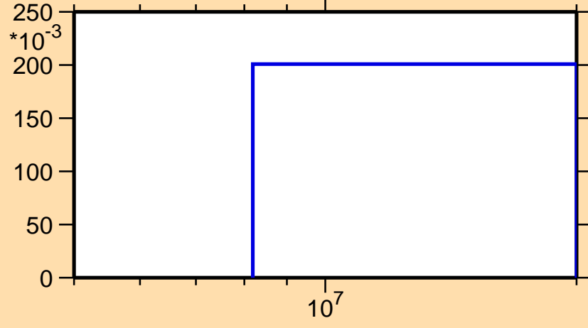
\sigma vs. E for ^{119}\text{I}(n,2n)
