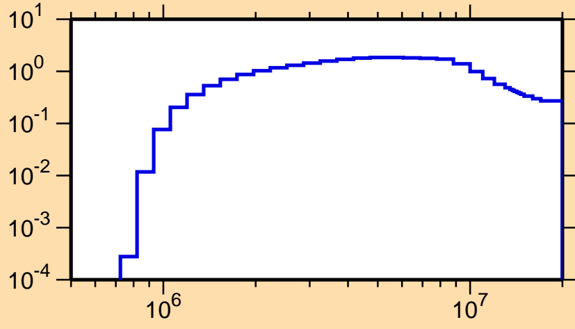
\sigma vs. E for ^{120}\text{I}(n,n\text{cont.})
